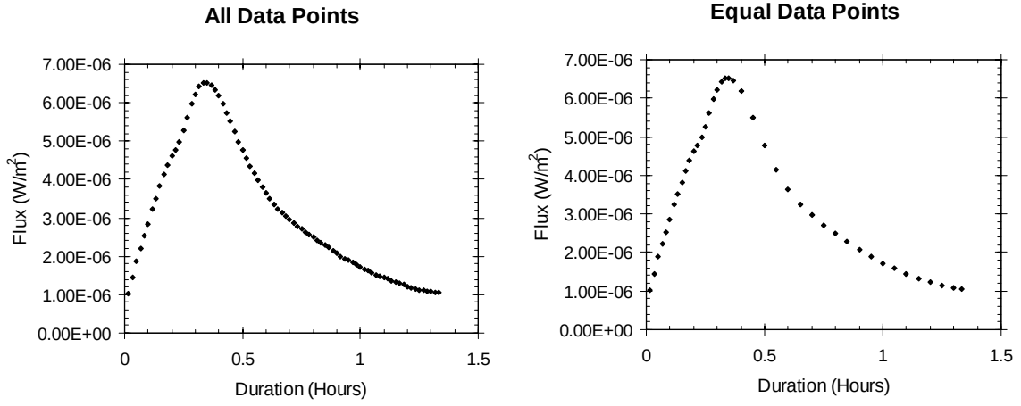
Figure 12. A C6 flare, from 27 May 2003, that had a total of 80 data points, 21 on the rise and 60 on the decay. The plot on the left shows all 80 points. The plot on the right shows the equally spaced data points used to calculate the RMSE and standard deviation.
