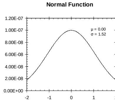
Figure 3. A normal function with a mean of 0.00 and a standard deviation of 1.52.
