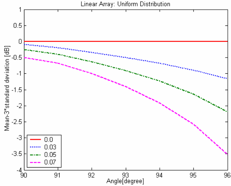
Figure. 3: Normalized EIRP degradation with n = 3 for uniform perturbation with different bounds of \Delta_{x \text{ and } y} = 0.0, 0.03, 0.05, \text{ and } 0.07 [m].
