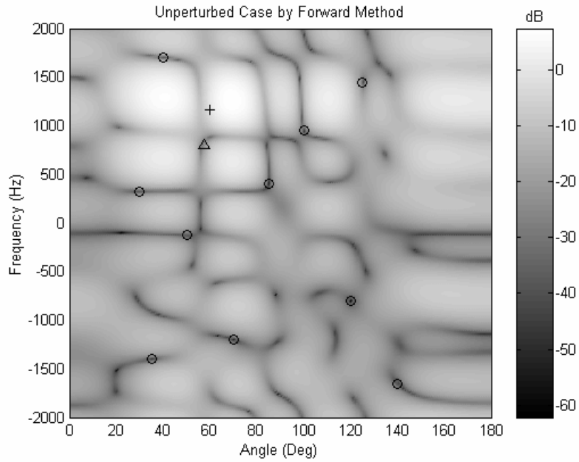
Figure. 6: Weight Spectrum of the Forward Method for the unperturbed case.
