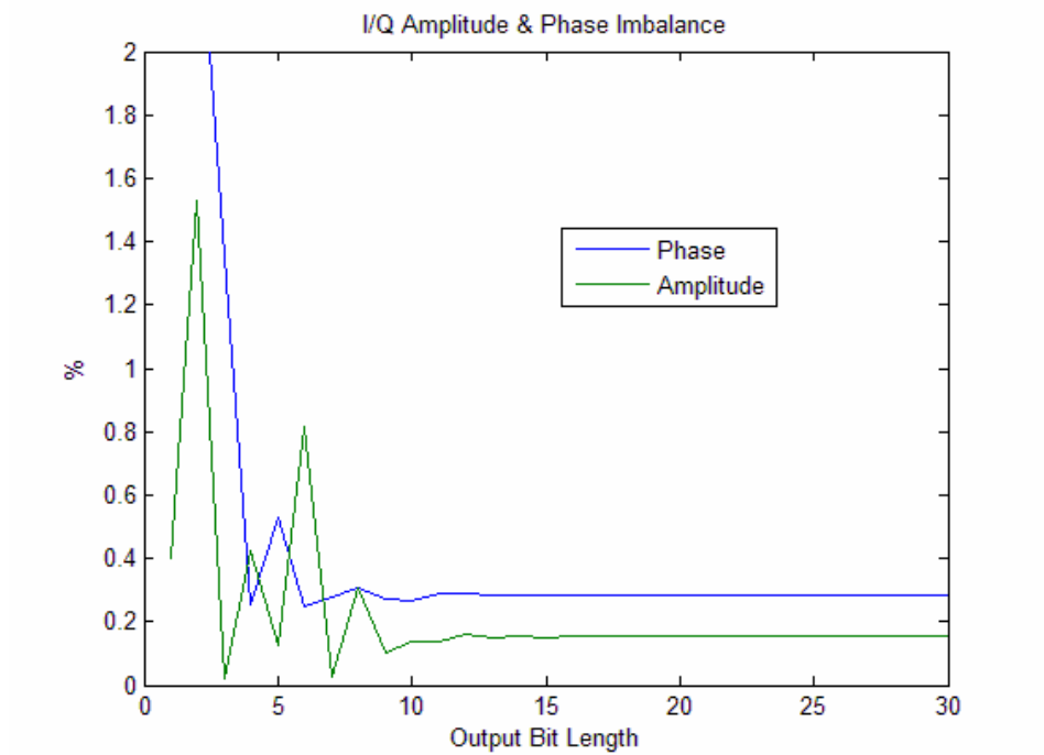
Figure 4.3: Imbalances of output bit-width at f_i = 14 MHz, f_s = 100 MHz.
