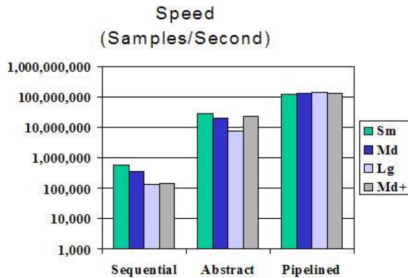
Figure 4.13: Circuit speed results using Cadence design synthesis flow for 0.25 um technology.
