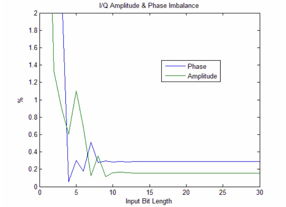
Figure 4.2: Imbalances of input bit-width at f_i = 7 MHz, f_s = 50 MHz.
