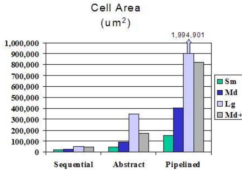
Figure 4.12: Circuit size results using Cadence design synthesis flow for 0.25 um technology.
