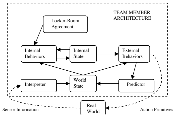
Figure 2.2: A functional input/output model of the CMUnited team member agent architecture [32].
