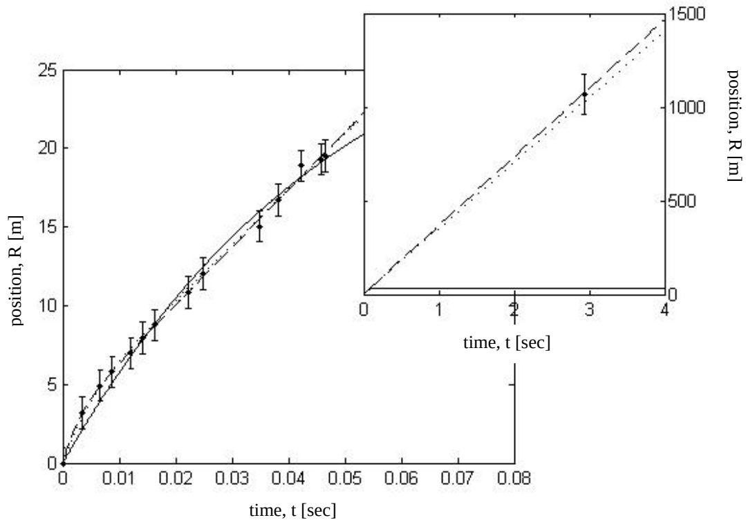
Figure 31: Position of the shockfront ( \bullet ) is shown with its uncertainty for an erect 155mm TNT detonation. The drag fit (solid line), modified drag fit (dashed line), and drag 350 fit (dotted line) are also shown. The functions were fit to the early-time data (lower left) with the late-time data point used to evaluate the fits in the far-field (upper right).
