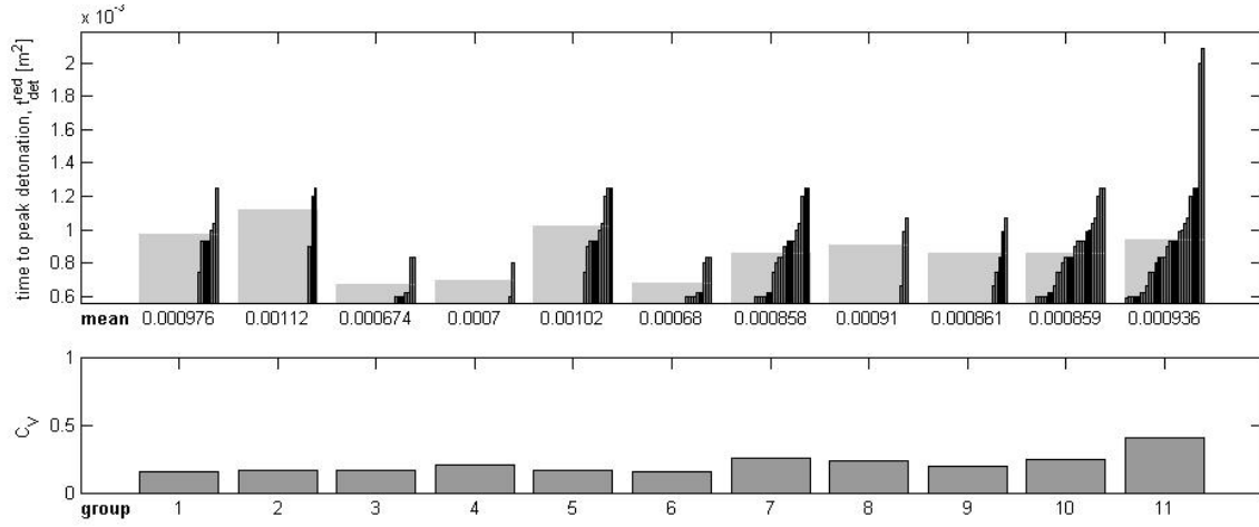
Figure 26: The time to the peak detonation area in the red band is shown for each event (thin bars) of the eleven munitions groups. The mean feature value is also shown for each group (wide bars) and the value is indicated below the top plot. The bottom plot shows the coefficient of variation for the feature in each group. t_{det}^{red} is a very reproducible feature for all groups, indicating it may be a feature common to explosives in general.
