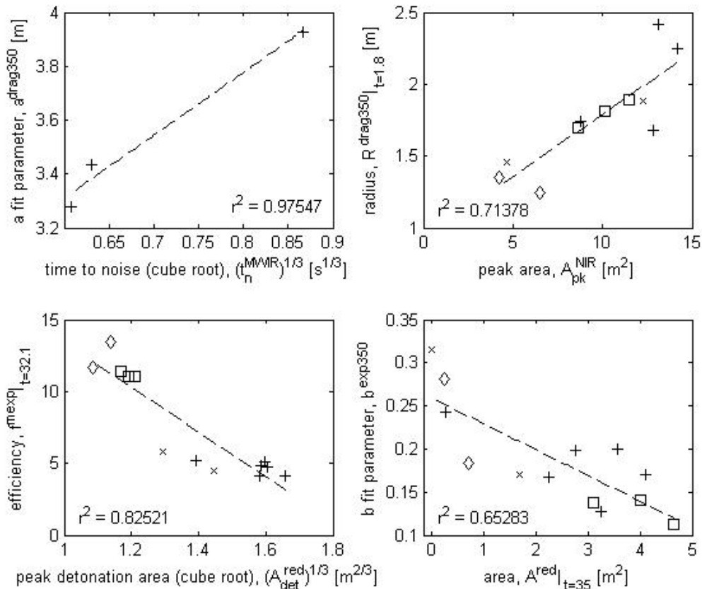
Figure 52: Selected comparisons of fireball and shockwave features are shown for TNT detonations only. The correlation between the features is the highest when only a single explosive composition is used and there are very clear trends.
