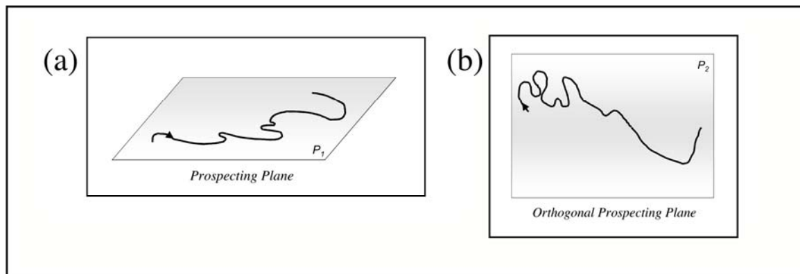
Figure 3.3. Prospecting planes in R&D innovation space. (a) an example plane P_1 ; and, (b) a prospecting plane P_2 that is orthogonal to plane P_1 .
