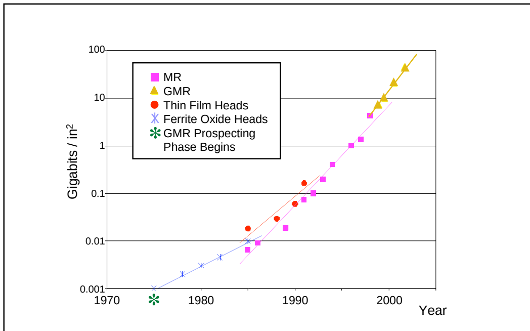
Figure 3.9. Magnetic Storage Density (Gigabits / in 2 ).
