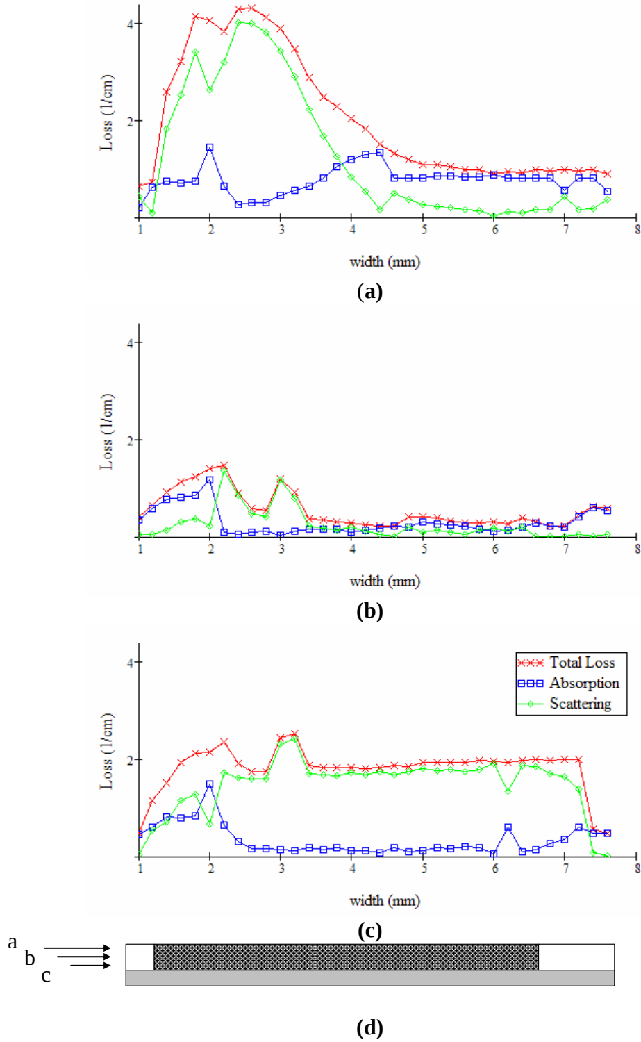
Figure 18: Sample 1 losses. (a) 480-μm from substrate, (b) 280-μm from substrate (c) 80-μm from substrate and (d) scaled end-view of sample depicting patterned areas and non-patterned areas.
