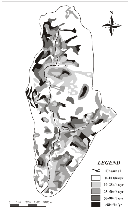
Figure 1. Soil loss map showing general distribution of soil erosion in Taipingxi watershed
