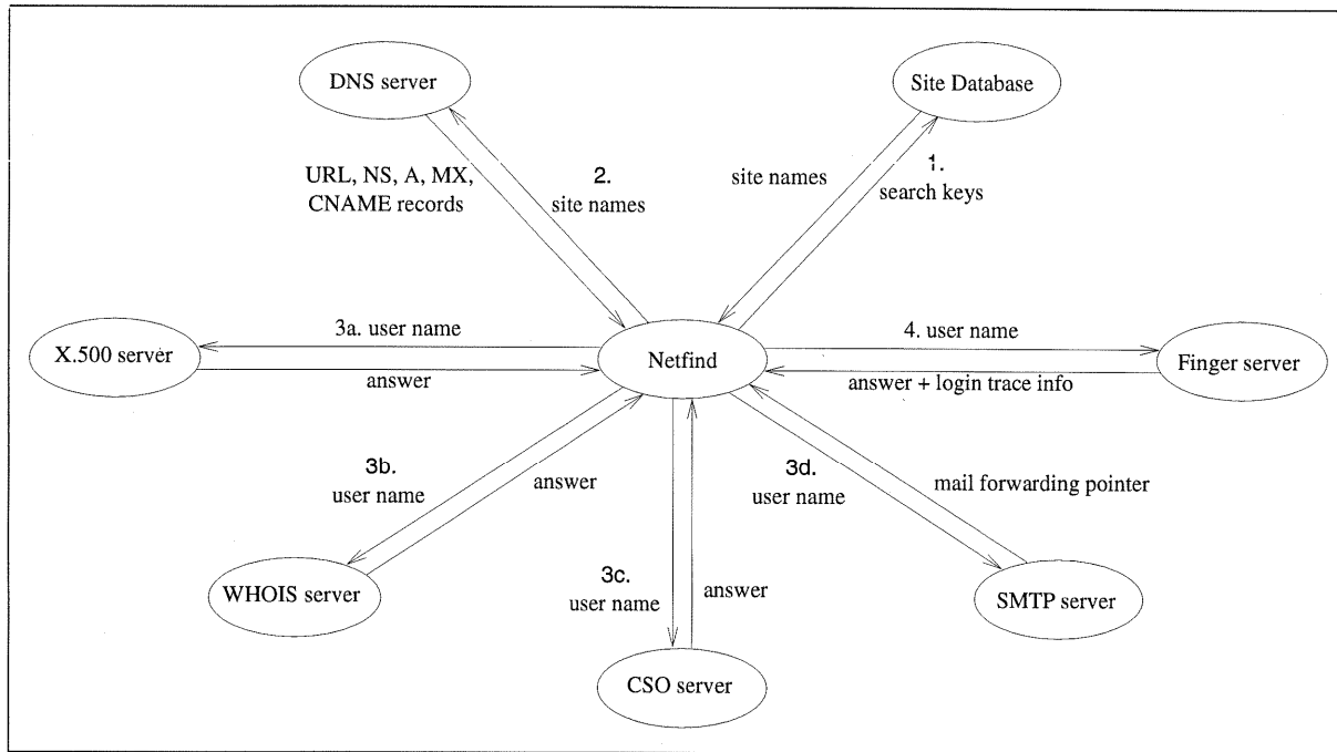
Figure 8: User Search Algorithm
