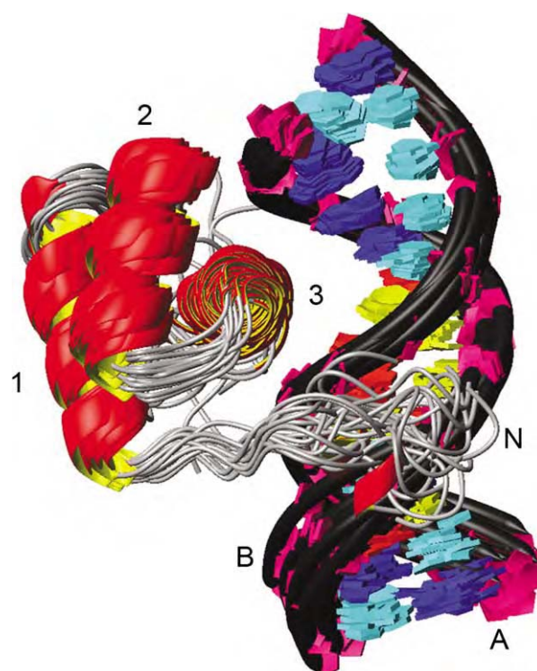
Figure 3. Superimposed ensemble of the 20 lowest energy structures from the AMBER docking calculation. Helices 1, 2, and 3, and the N terminus of the homeodomain are labeled. The sense and anti-sense strands are labeled A and B, respectively. Cytosine (cyan), guanosine (blue), thymine (yellow), and adenine (red) bases, deoxyribose sugars (magenta), and the phosphate backbone (black) are color-coded. Helix 3 inserts into the major groove and the N-terminal arm wraps around and contacts the minor groove. Statistics for the ensemble are given in Table 1.
