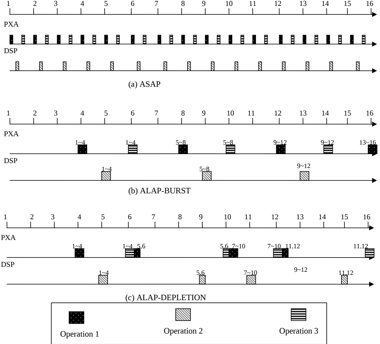
Figure 8 Comparison of heuristic scheduling algorithms
