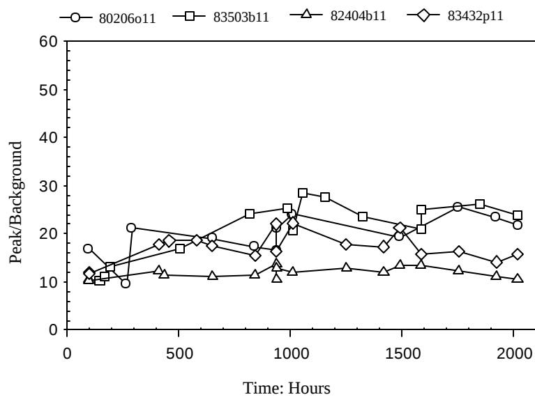
Figure 6. \text{HgI}_2 Life Tests: Ambient Conditions. Composite Graph of Four \text{HgI}_2 Detectors. ^{137}\text{Cs} ; Peak/Background Ratio; Area = 100 mm 2 ; 24 \mu\text{sec} Amplifier Shaping Time.
