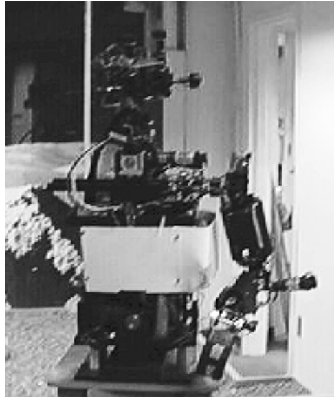
Figure 1: Cog, an upper-torso humanoid robot. Cog has two degrees-of-freedom in the waist, one in the shoulder, three in the neck, six on the arm, and two for each eye.
