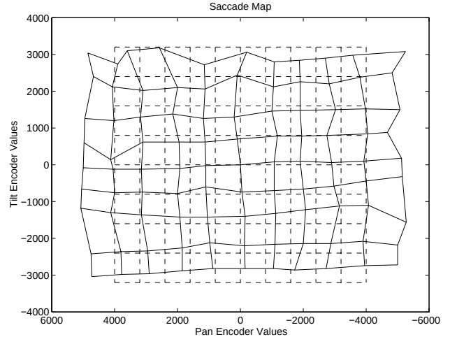
Figure 4: Saccade Map after 0 (dashed lines) and 2000 (solid lines) learning trials. The figure shows the pan and tilt encoder values for every tenth position in the image array within the ranges x=[10,110] (pan) and y=[20,100] (tilt).
