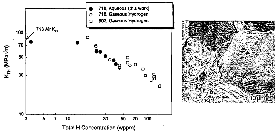
Figure 2. Threshold stress intensity for HEAC in peak aged IN718 and IN903, stressed in high pressure H_2 (9, ○) or acidified chloride solution with cathodic polarization (●), vs. calculated H content produced at the crack tip. H-free superalloys cracked by microvoid processes at high K_{IC} , while HEAC in each environment produced mixed IG and TG slip-plane based cracking, as shown in the SEM fractograph (IN718 at K = 53 \text{ MPa}\sqrt{\text{m}} ) [12].
