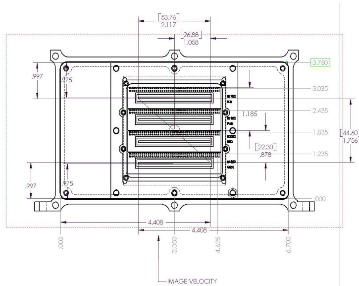
Figure 2 Geometrical layout of the four sensor arrays in the focal plane.
