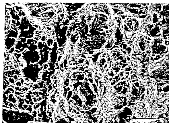
FIGURE 4. Scanning electron image of the fracture surface of hydrogen-charged Fe-13Co-11Ni-3Cr-1Mo-0.2C steel after baking at 190^{\circ}\text{C} for 24 hours. The specimen was previously charged to a diffusible H concentration of 4.6 wppm.
