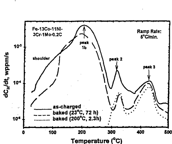
FIGURE 5. H desorption rate as a function of temperature for peakaged Fe-13Co-11Ni-3Cr-1Mo-0.2C steel, measured by TDS at a ramp heating rate of 5°C/min, showing the effect of baking compared with the as-charged condition (charged at overpotential of -0.62 V at 60°C). 36
