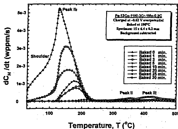
FIGURE 8. Hydrogen desorption rates versus TDS ramp temperature for H precharged and baked uncoated Fe-13Co-11Ni-3Cr-1Mo-0.2C steel specimens after the indicated baking times at 190°C. TDS tested at dT/dt = 5 °C. Charging was performed in saturated \text{Ca}(\text{OH})_2 .
