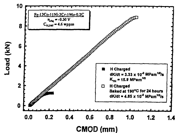
FIGURE 3. Load versus CMOD data for H precharged ( C_{H,Diff} = 4.6 \text{ wppm} ) and precharged/baked Fe-13Co-11Ni-3Cr-1Mo-0.2C steel. Charging was conducted in saturated \text{Ca}(\text{OH})_2 at overpotential of -0.30 \text{ V} at 60^{\circ}\text{C} for 20 days. Baking was performed at 190^{\circ}\text{C} for 24 hours. 15
