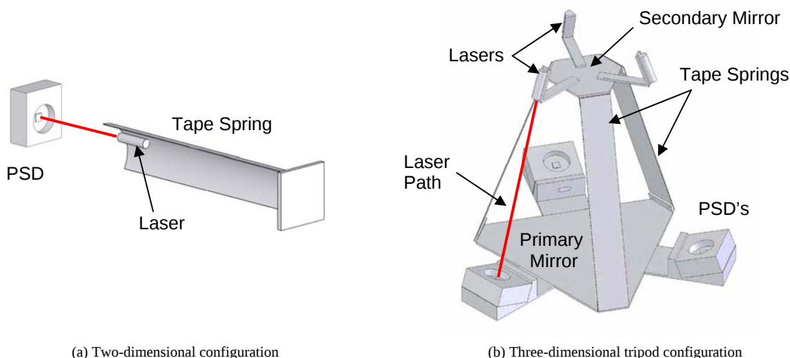
Figure 2 – Experiment configuration for 2D and 3D tests
