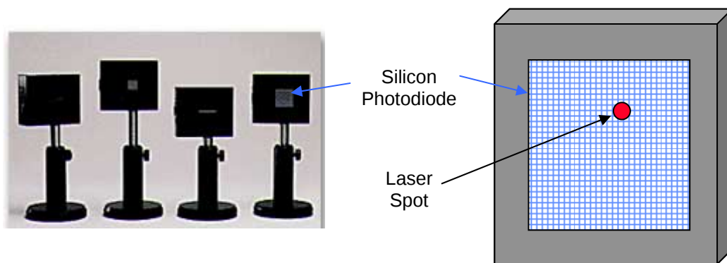
Figure 1 – On-Trak position sensing detectors (PSD's) along with notional diagram
