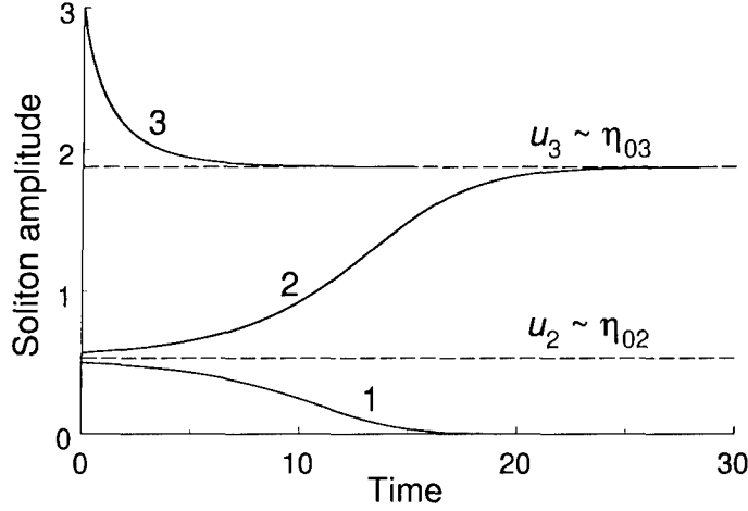
Figure 8: Soliton amplitude versus time in dimensionless variables as given by Eq. (70) for three different initial conditions ( 1 - u_0 = 0.5 ; 2 - u_0 = 0.57 and 3 - u_0 = 3.0 ). Normalized variables are: u = \eta_0 \frac{\alpha \delta_t}{15\beta\epsilon} , \tau = 4\epsilon t/3 , \gamma = 2.1 .
