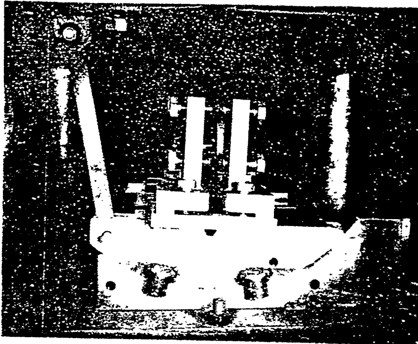
Figure 16 Modified Clamping Unit for Rocker End
