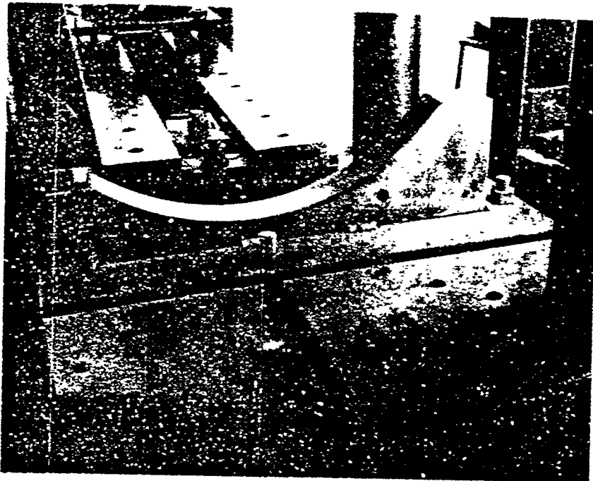
Figure 17 Track Shown Mounted on Lower Platen of Press
