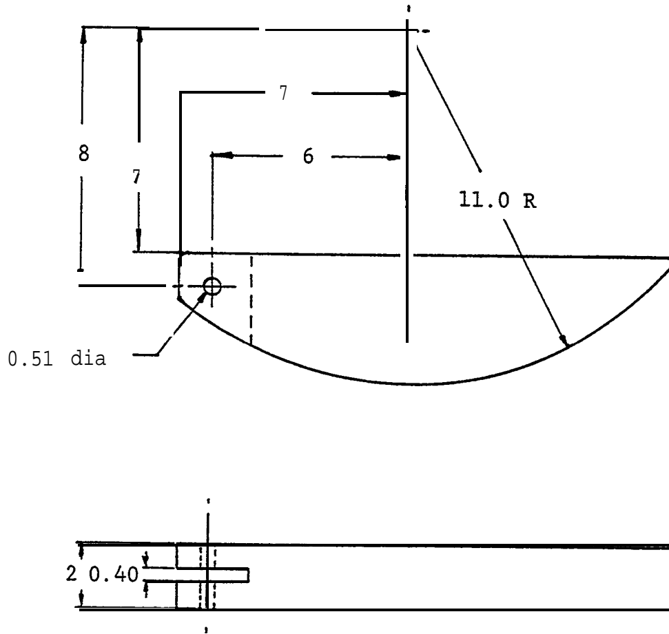
Figure 8 Rocker
