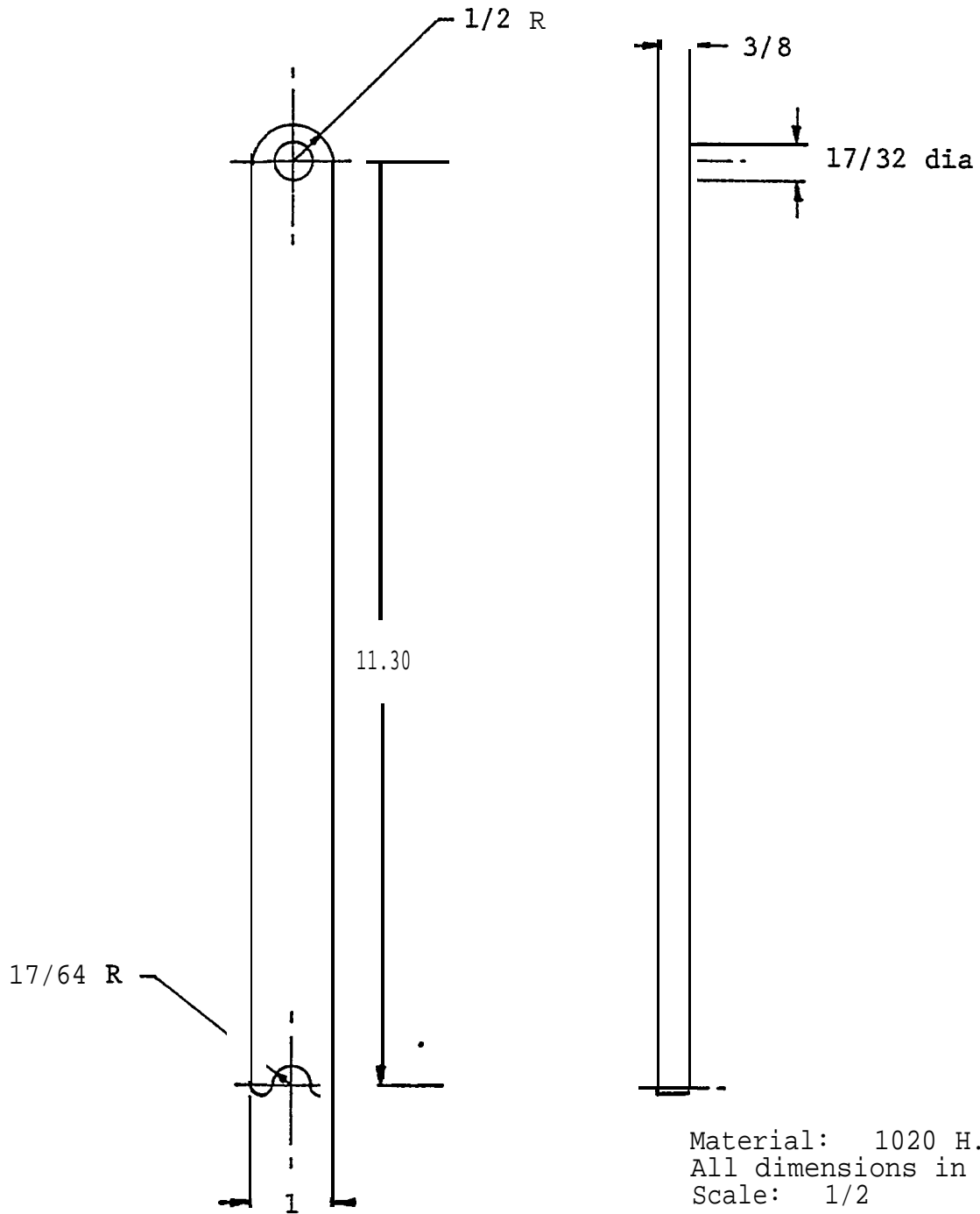
Figure 9 Coupler Bar
