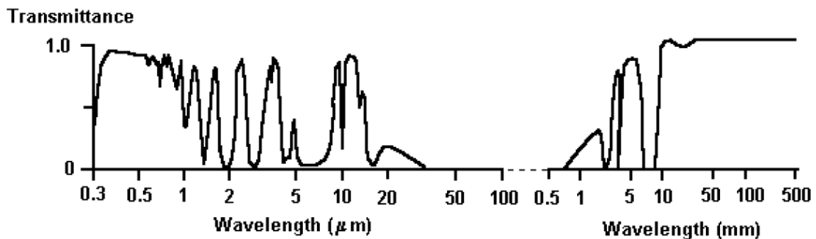
Figure 14. The wavelength "windows" generally used in remote sensing are defined by narrow spectral absorption bands.
