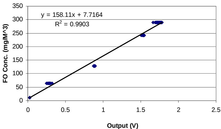
Figure 12. Linear regression calibration of RAS-4.
