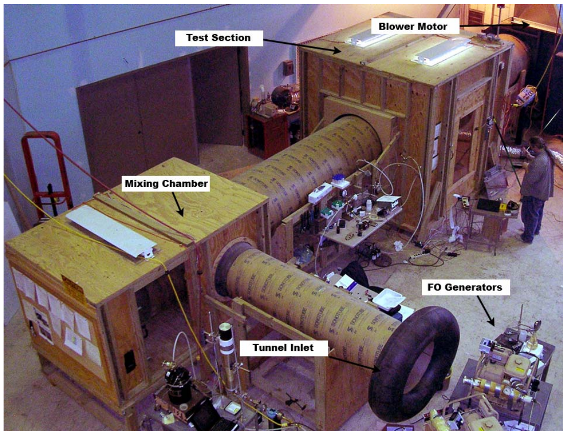
Figure 6. Open jet wind tunnel view from above.
