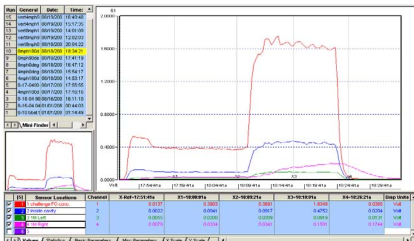
Figure B-6. FO concentration profile for model tree trunk cavity testing at 8 mph, 180 degrees, 2 concentrations (60 mg/m³ and 250 mg/m³).
