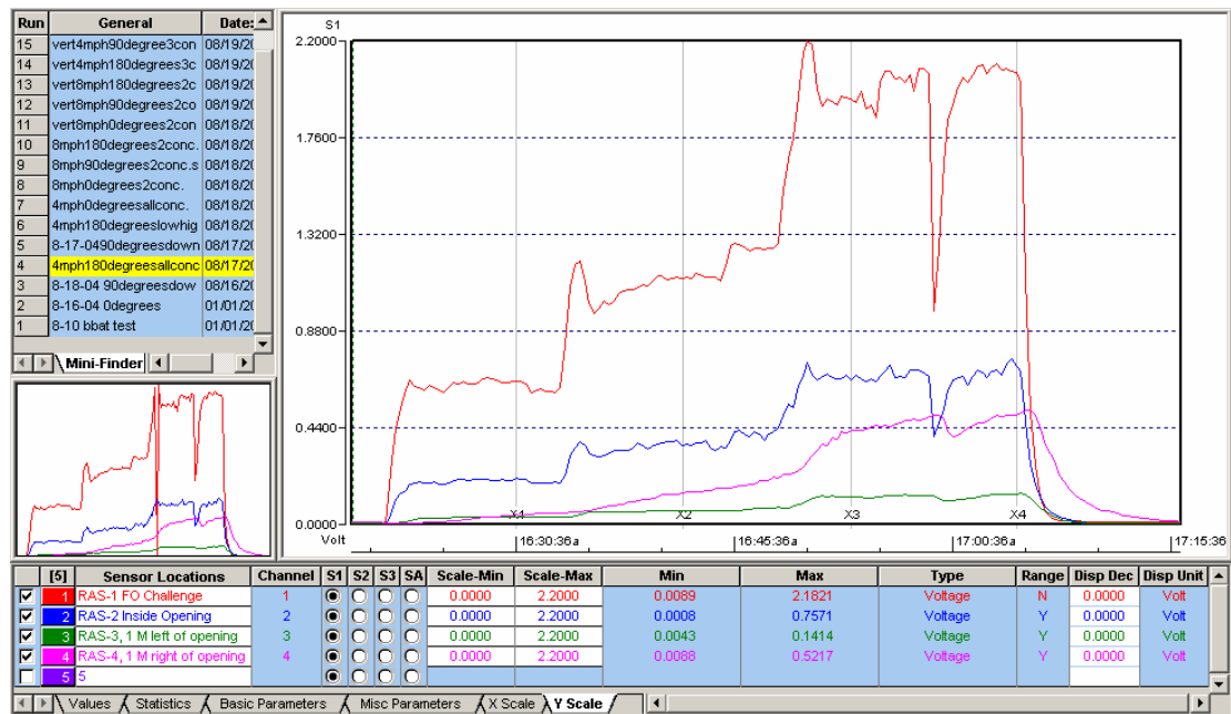
Figure B-3. FO concentration profile for model tree trunk cavity testing at 4 mph, 180 degrees, 3 concentrations.
