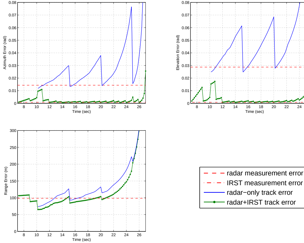
Figure 5: Track error for the straight missile trajectory
