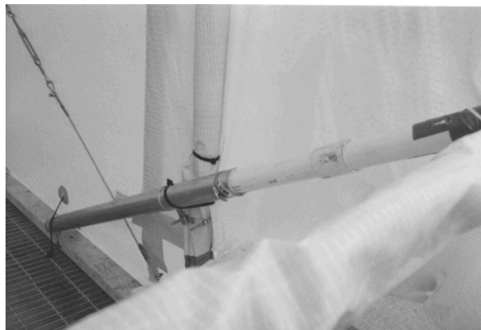
Figure 12: Piston Arrangement Used to Help Place Membrane Seals Against Vessel
