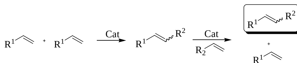
Scheme 1-10. Primary and secondary CM metathesis reactions
