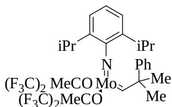
Schrock's catalyst 1-1
