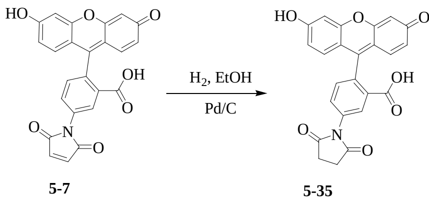
Scheme 5-13: Hydrogenation of fluorescein maleimide 5-7 .
