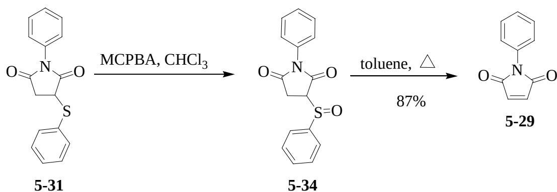
Scheme 5-12. Oxidation and elimination reactions
