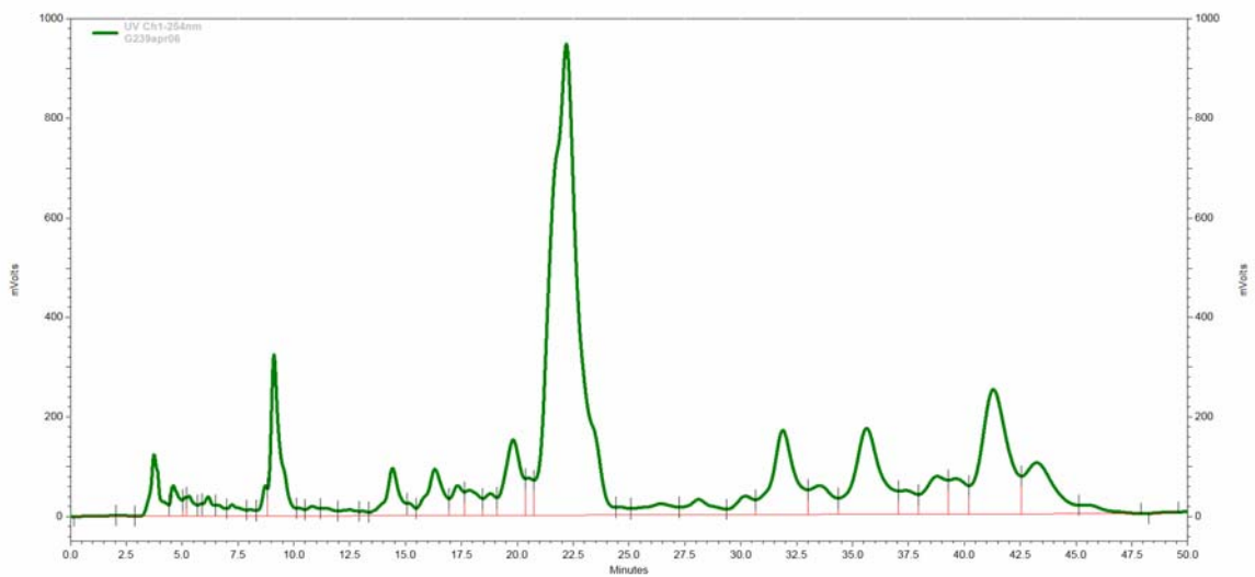
Figure A-10. HPLC spectrum of Experiment 13 reaction mixture ( \text{CH}_2\text{Cl}_2 , 5mM, Reflux 15 hours, LiI)
