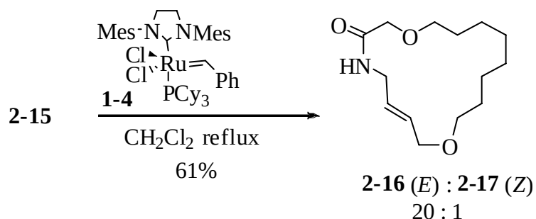
Scheme 2-6. RCM of 2-15
