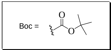
Scheme 3-3. Synthesis of trimer scaffold
