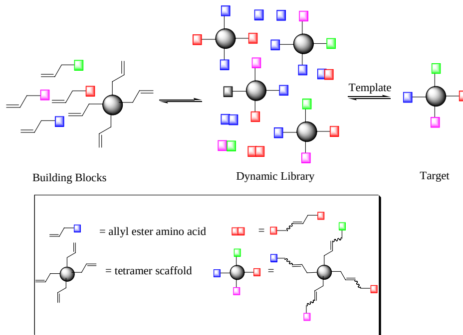
Figure 3-10. Dynamic library of cyclic tetrapeptidomimetics
