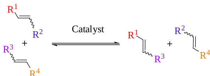
Scheme 1-1. Olefin metathesis
