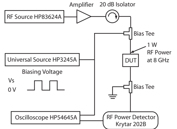
Fig. 9. Switching speed and reliability measurement test setup.
