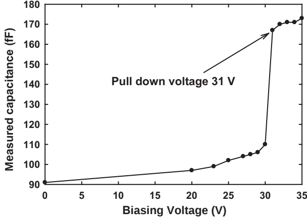
Fig. 6. Measured capacitance vs. voltage curve of a 1-port switched capacitor.
