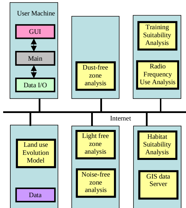
Figure 7. Software plan for the sustainability, encroachment, and room to maneuver program.
