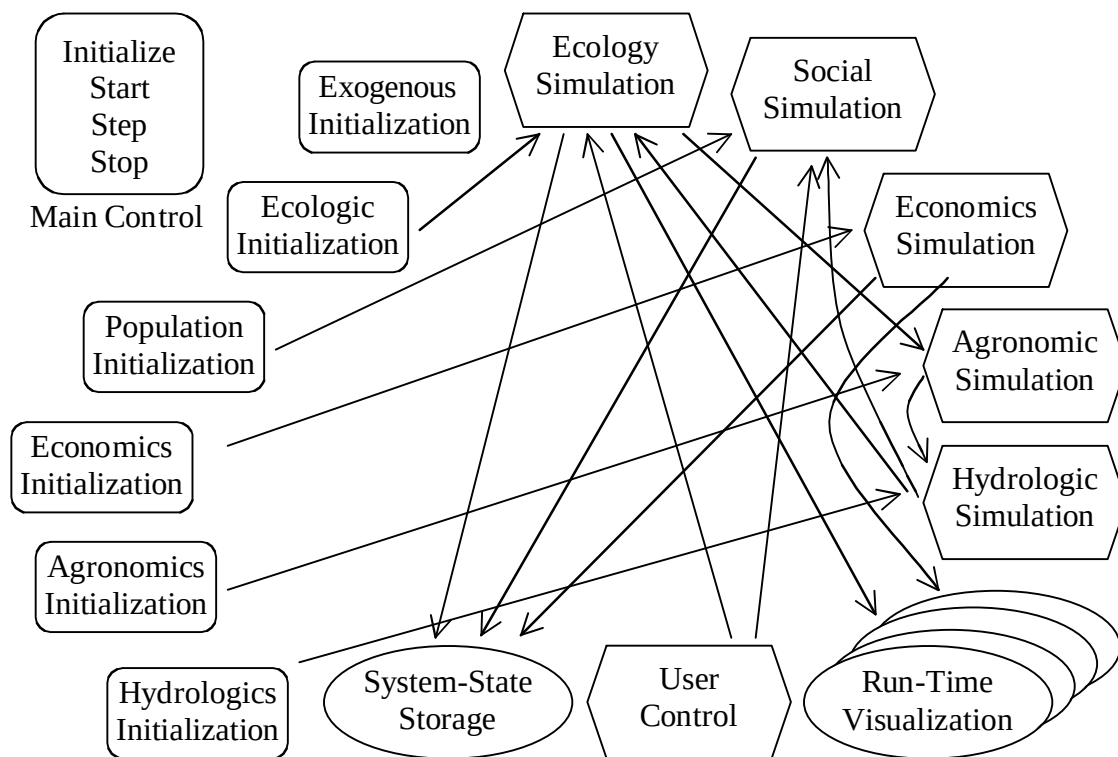
Figure 8. A services centric view.
