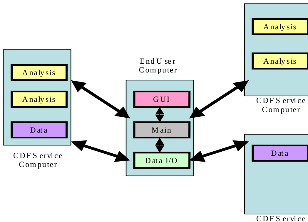
Figure 4. Delivery of Internet service software example.
