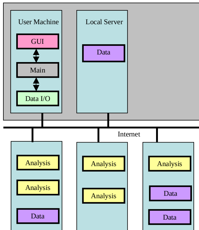
Figure 5. Combining desktop/local, and distributed services.
