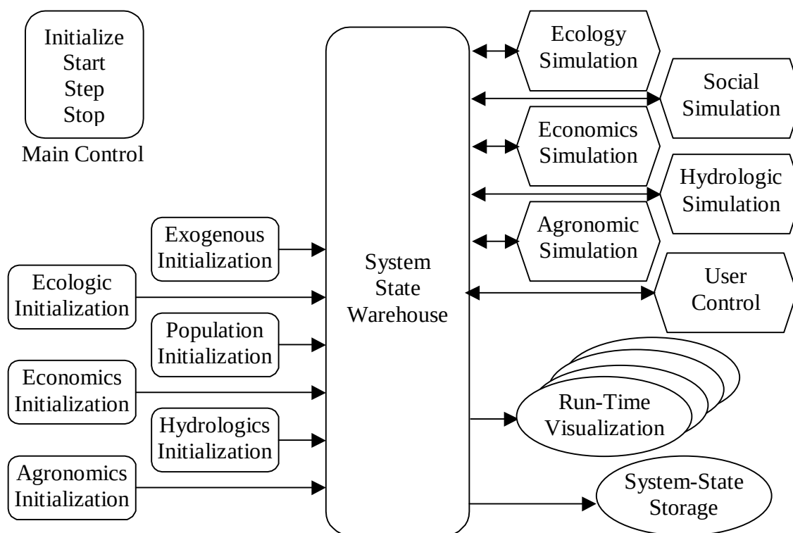
Figure 9. A system state centric approach.
