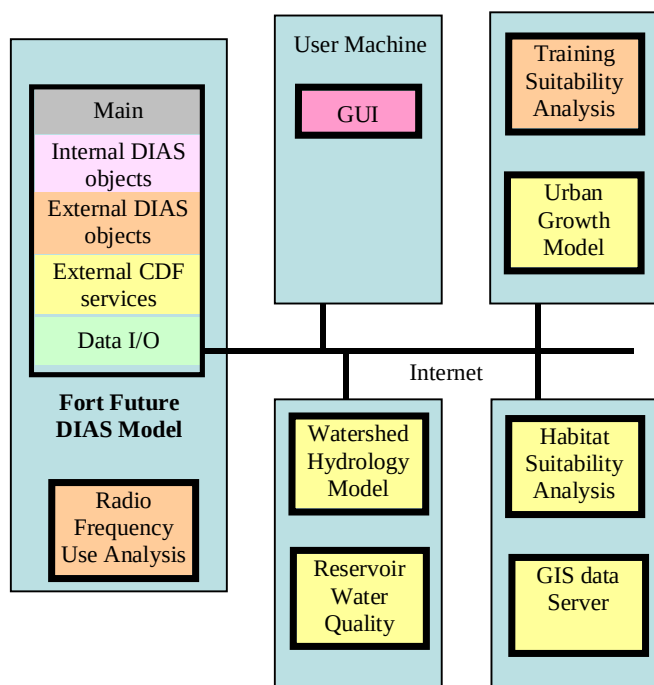
Figure 10. A Fort Future DIAS model.
