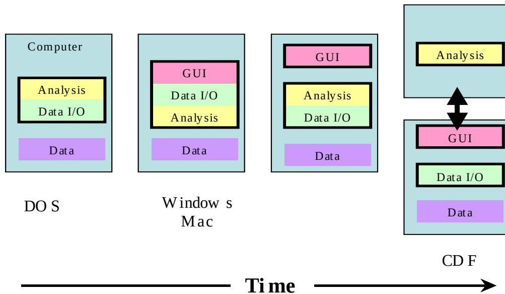
Figure 3. Historic software designs.
