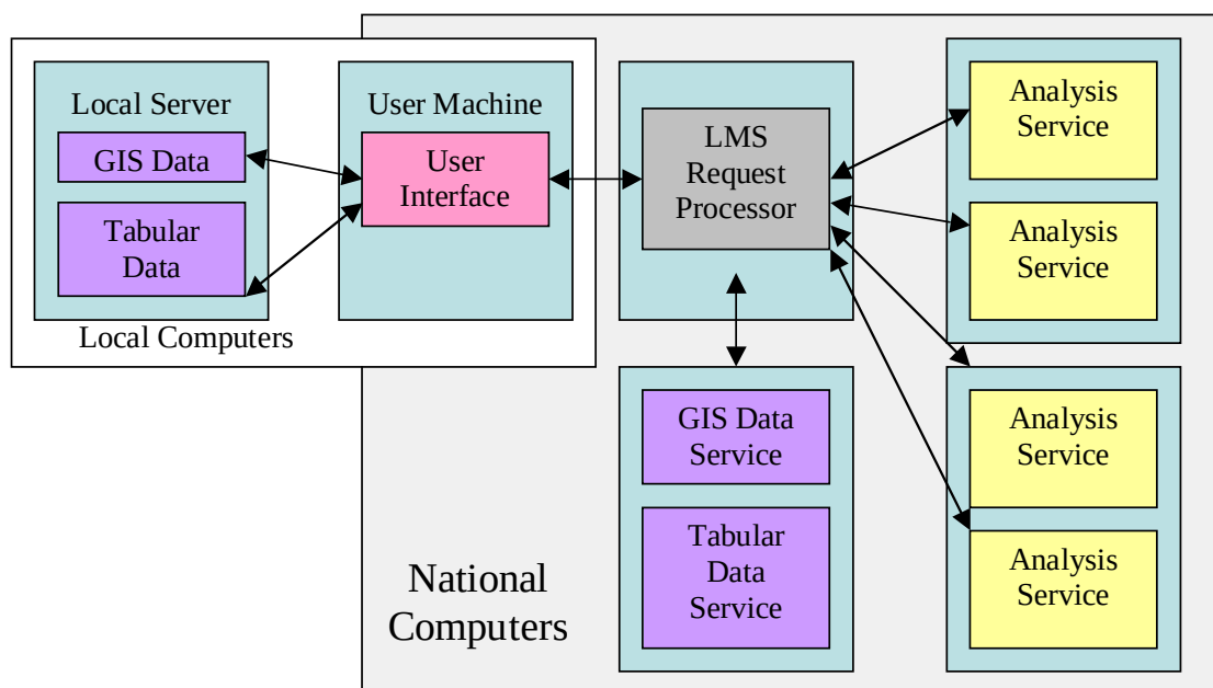
Figure 6. Land management suite gross architecture.
