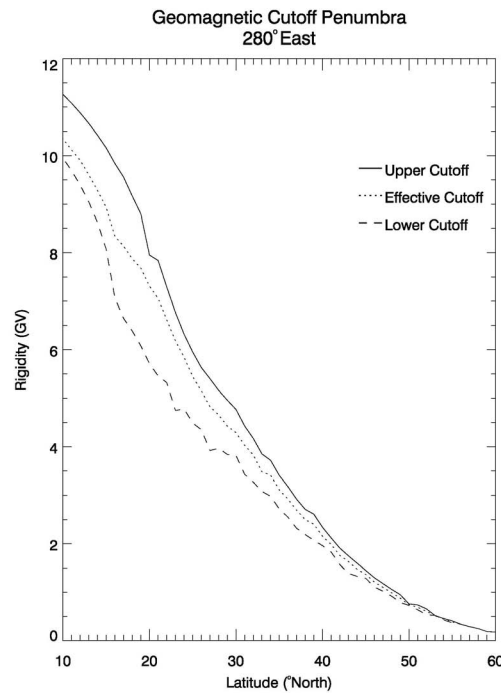
Figure 20: Geomagnetic cutoff penumbra along the 280° East meridian. Note that the size of the penumbra increases as latitude decreases and rigidity increases. Below approximately 1 GV in rigidity, or higher than 50° in latitude, the cutoff penumbra decreases rapidly in width.
