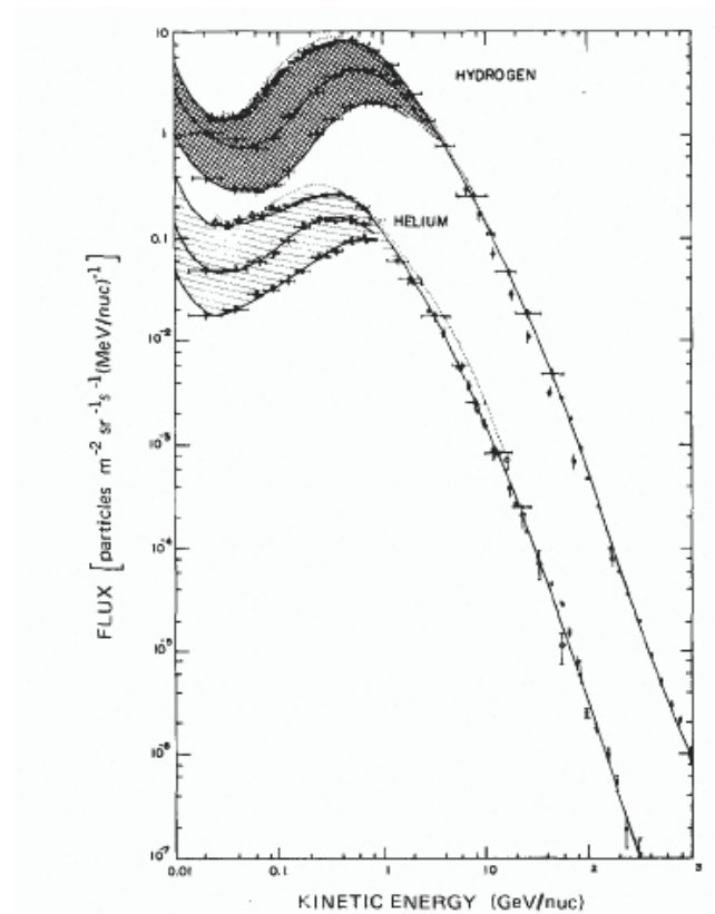
Figure 2: Primary cosmic ray differential energy spectra for helium and hydrogen shown on a log scale. The shaded areas are those regions where the spectra deviate from the power law and are affected by solar activity. The upper/lower bound is a solar minimum/maximum spectrum. The hydrogen spectrum has been multiplied by a factor of five so the lower portion of the spectrum avoids merging with the top of the helium spectrum (26:6-4).
