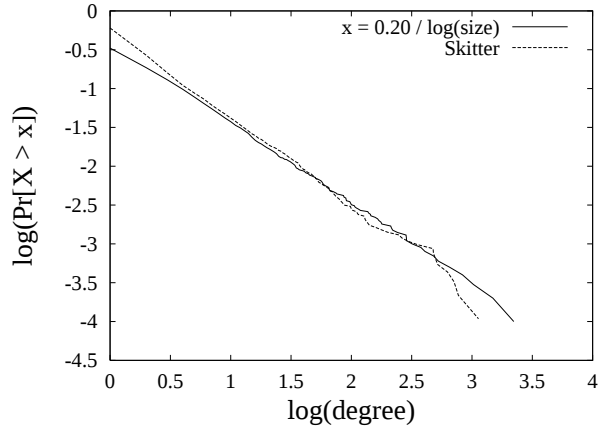
Figure 5: Diminishing Probability where x = 0.20 .
