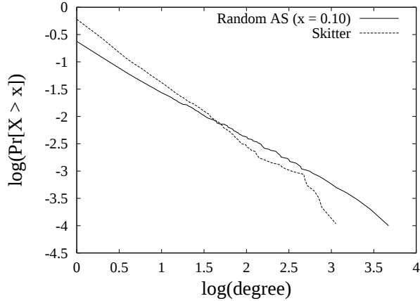
Figure 4: Predicted Degree Distribution where x = 0.10
