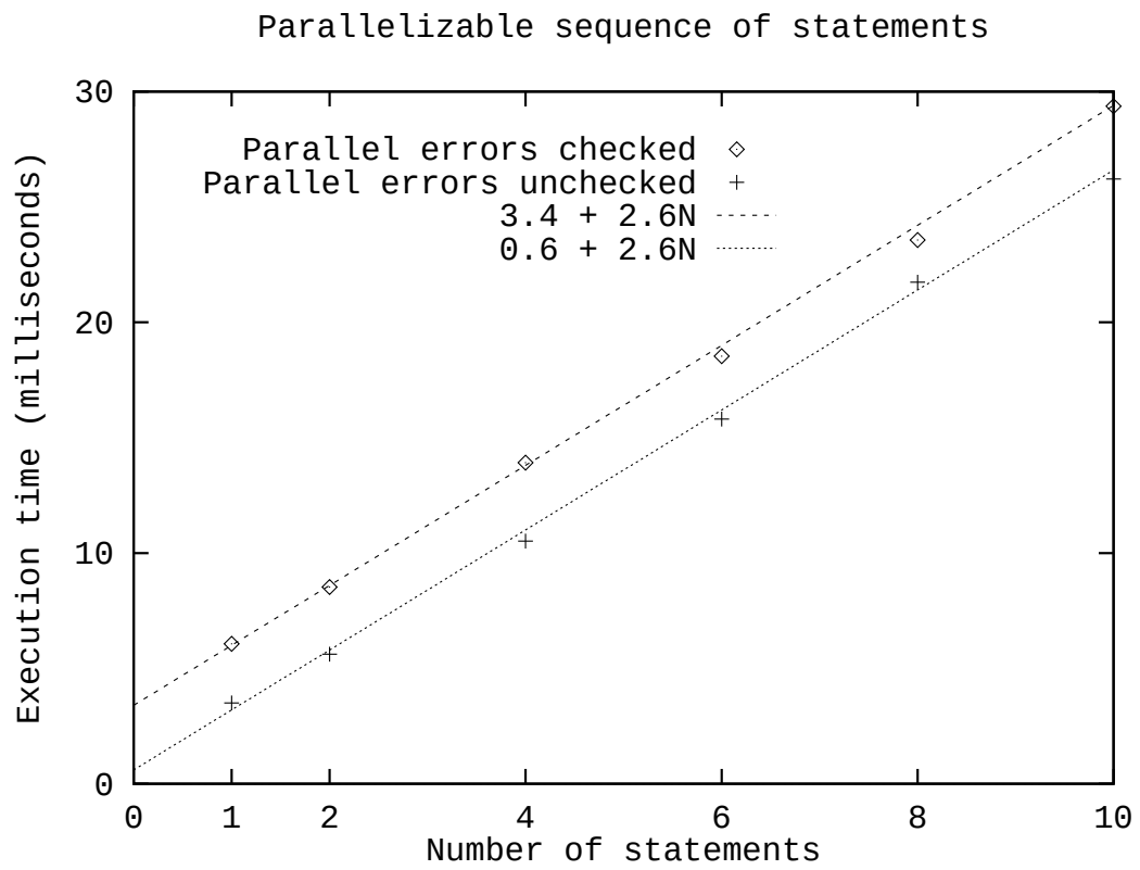
Figure 5.1: Execution time of a parallelizable sequence of statements on a single processor.
