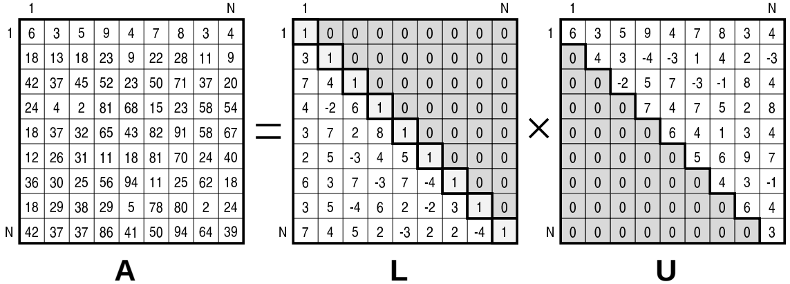
Figure 1.1: An example of LU factorization.
