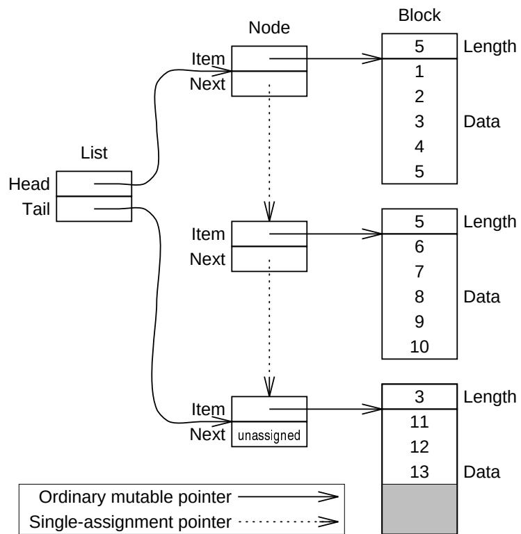
Figure 7.1: An example of a linked list of blocks of integers.
