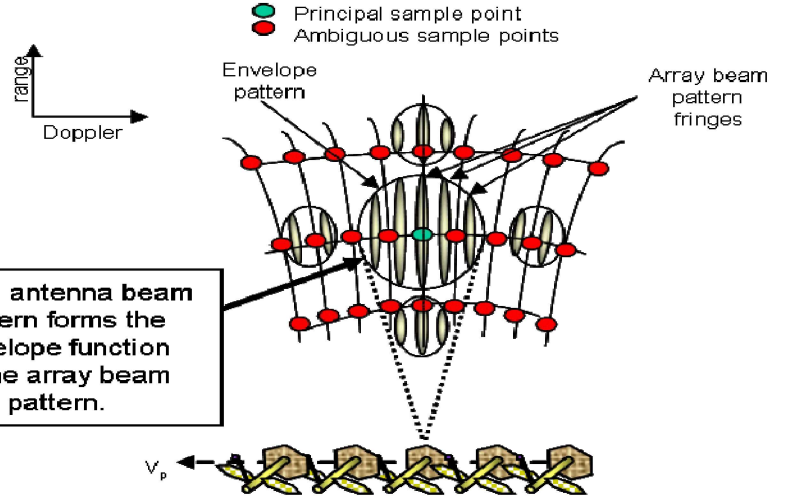
Figure 2. PRF sampling grid and antenna beam pattern.
