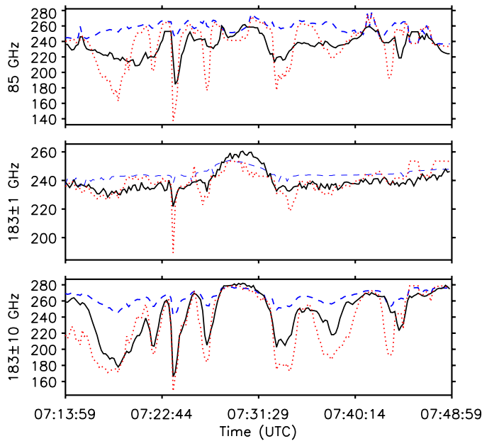
Figure 5. Comparisons between observations and frozen particles with a Sekhon-Srivastava PSD (red dotted line) and dry, low-density, large fluffy PSD (blue dashed line).
