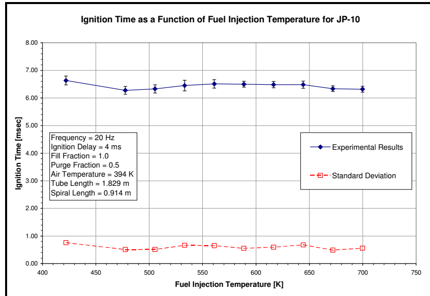
Figure 73. Ignition time as a function of fuel injection temperature for a JP-10/air mixture
