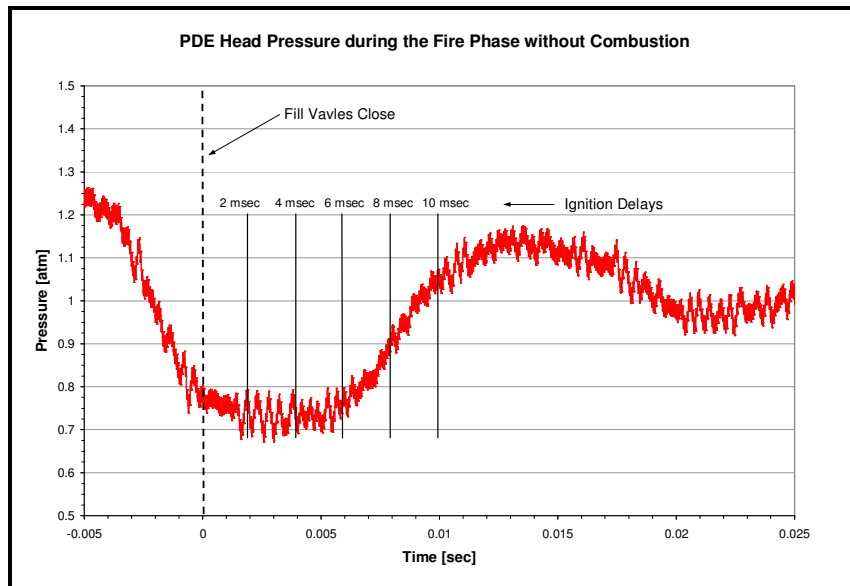
Figure 15. PDE head pressure during fire phase without combustion (vertical lines denote various spark delays)
