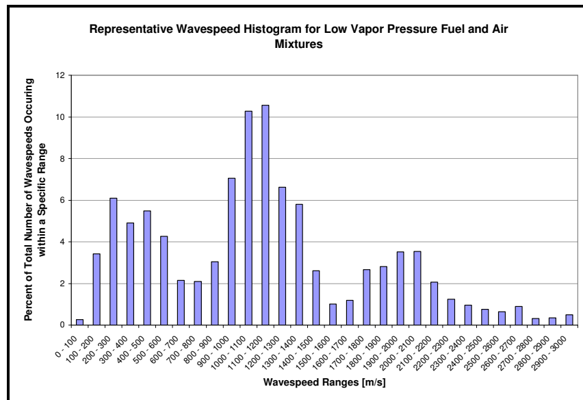
Figure 37. Representative wavespeed histogram for a low vapor pressure fuel and air mixture
