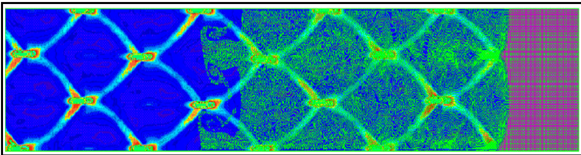
Figure 5. CFD smoke foil for two-dimensional H_2 /air mixture detonation cell structure (Katta, 1999)
