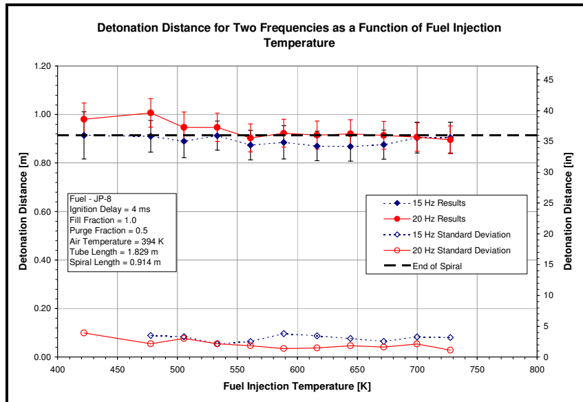
Figure 61. Comparison of detonation distance for two frequencies as a function of fuel injection temperature with a JP-8/air mixture with an ignition delay of 4 msec
