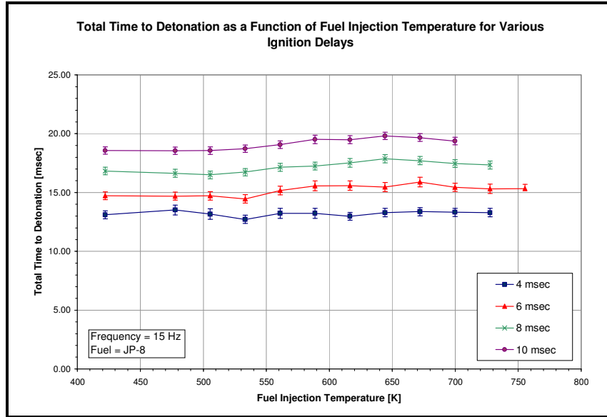
Figure 55. Total time to detonation for a JP-8/ari mixture as a function of fuel injection temperature for various ignition delays with a frequency of 15 Hz
