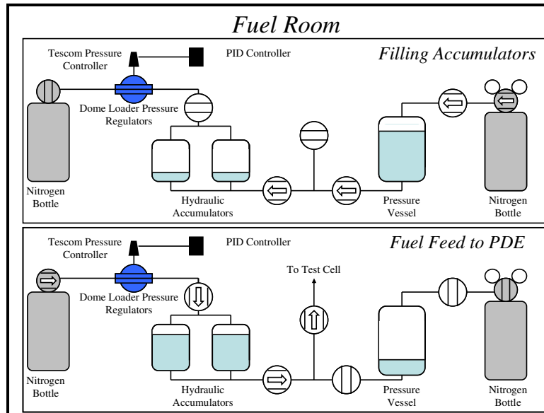
Figure 24. Schematic diagram of the liquid flow in the fuel room during both filling and testing
