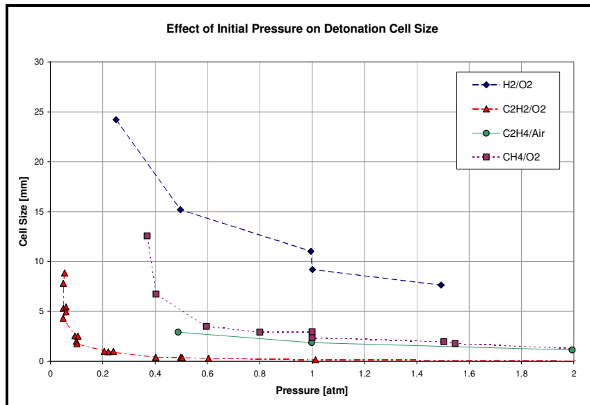
Figure 17. Effect of initial pressure on detonation cell size (Data from Kaneshiga, 1997)
