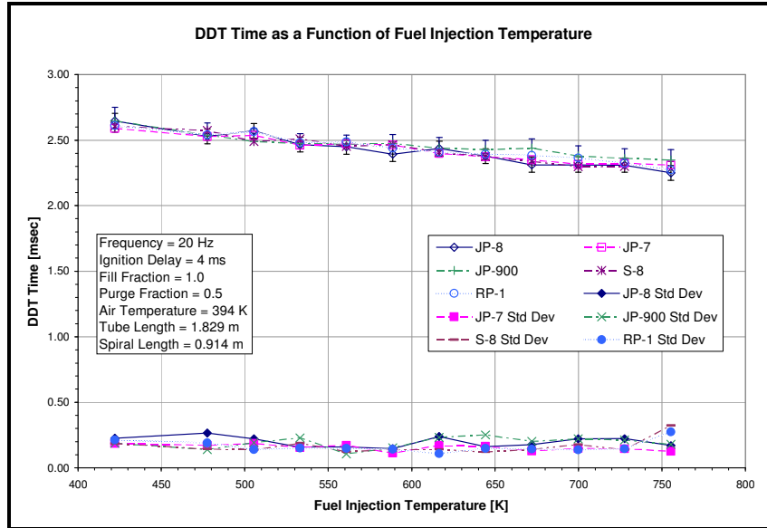
Figure 48. Comparison of the DDT time for five fuels as a function of fuel injection temperature with a frequency of 20 Hz and an ignition delay of 4 msec
