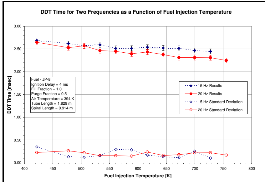
Figure 60. Comparison of DDT time for two frequencies as a function of fuel injection temperature with a JP-8/air mixture with an ignition delay of 4 msec
