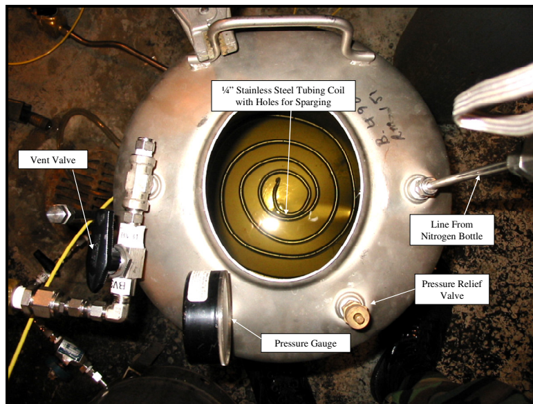
Figure 26. Photograph of the top view of fuel conditioning holding tank with nitrogen bubbling coiled tube at the tank bottom
