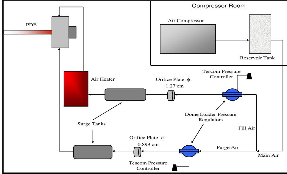
Figure 22. Diagram of PDE main air supply system
