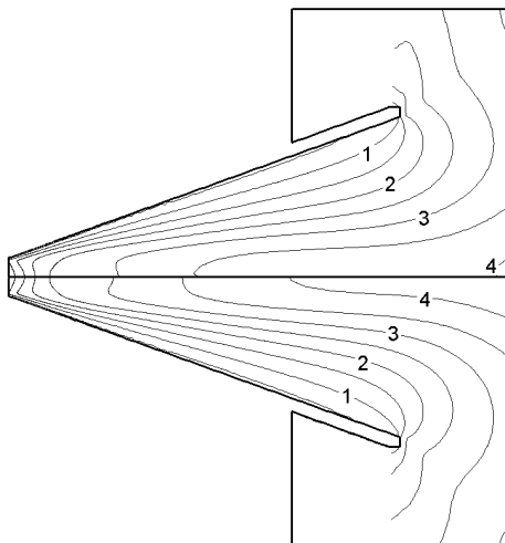
Fig. 3 Mach number contours for ES-BGK (top) and DSMC (bottom).
