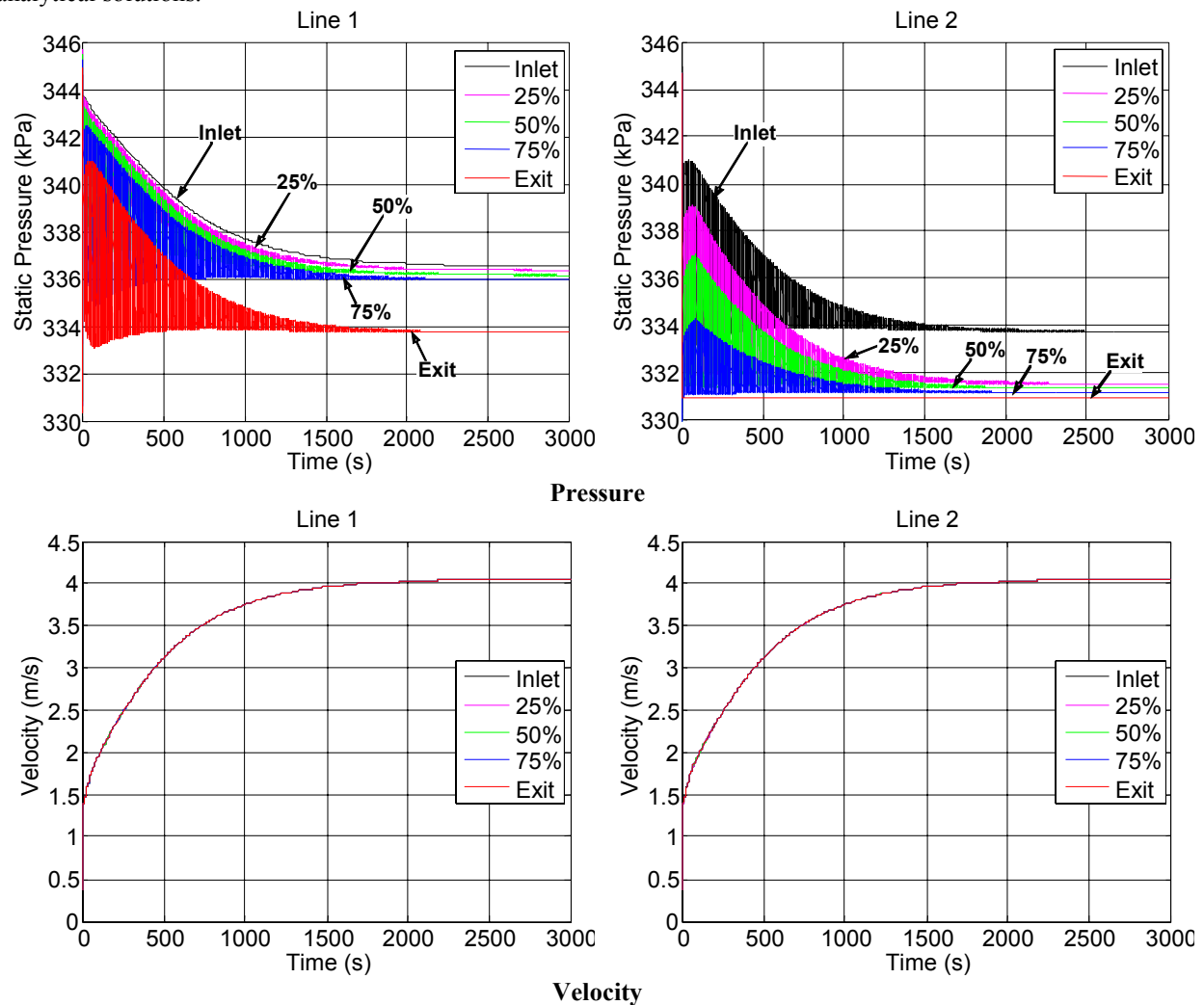
Figure 4. Water transient viscous pipe flow using point-implicit numerical technique.
