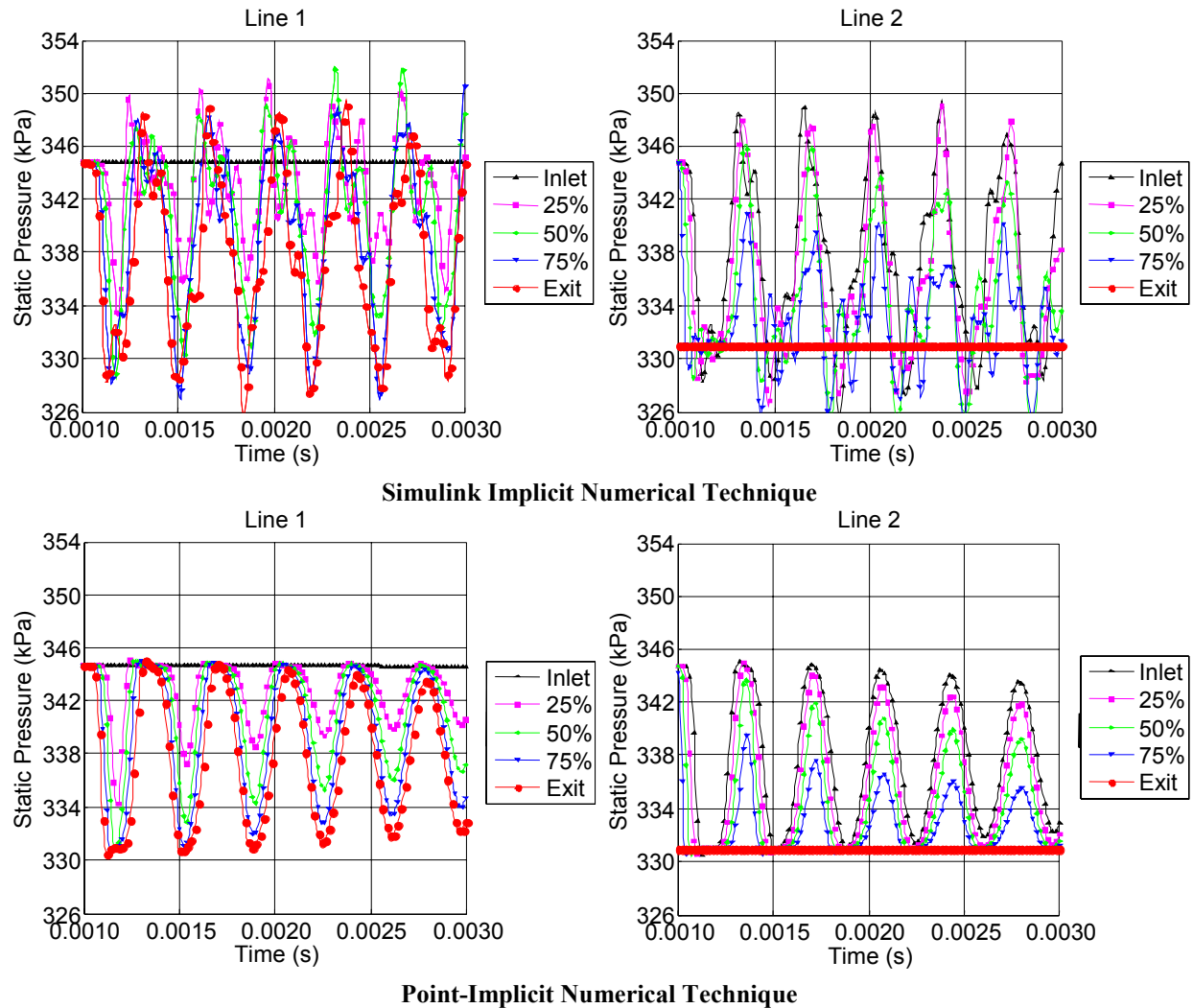
Figure 5. Transient pressure comparison of numerical techniques for water transient viscous pipe flow.
