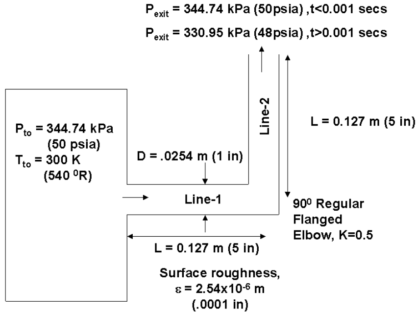
Figure 1. Two-pipe system.
