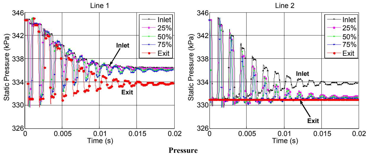
Figure 2. Nitrogen transient viscous pipe flow using explicit numerical technique.
