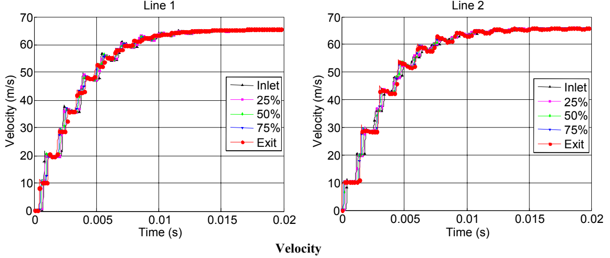
Figure 2. (cont) Nitrogen transient viscous pipe flow using explicit numerical technique.
