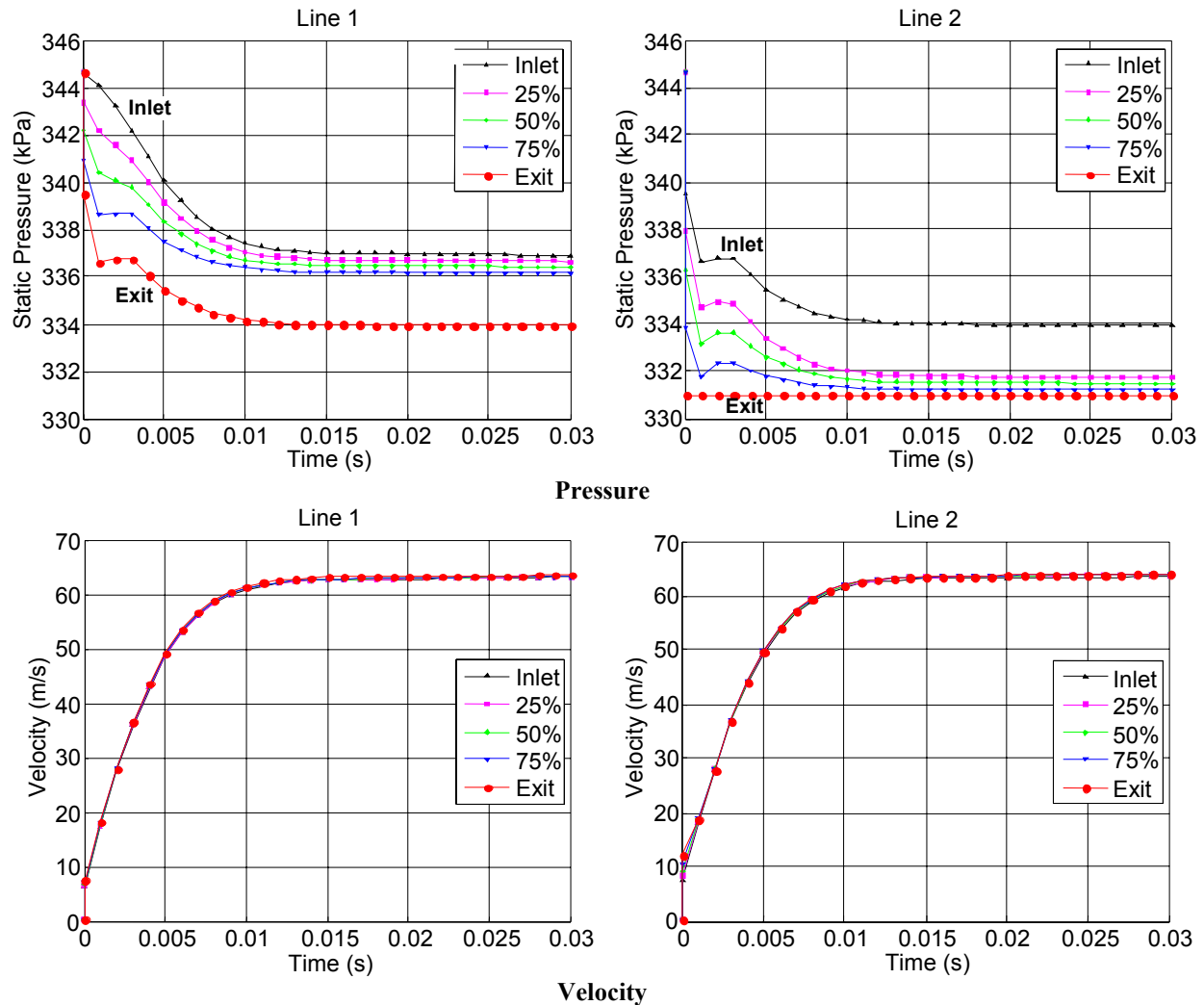
Figure 3. Nitrogen transient viscous pipe flow using point-implicit numerical technique.
