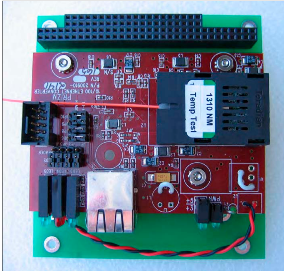
Figure I-3. Electro-optical converter and PC/104 card adapter.
