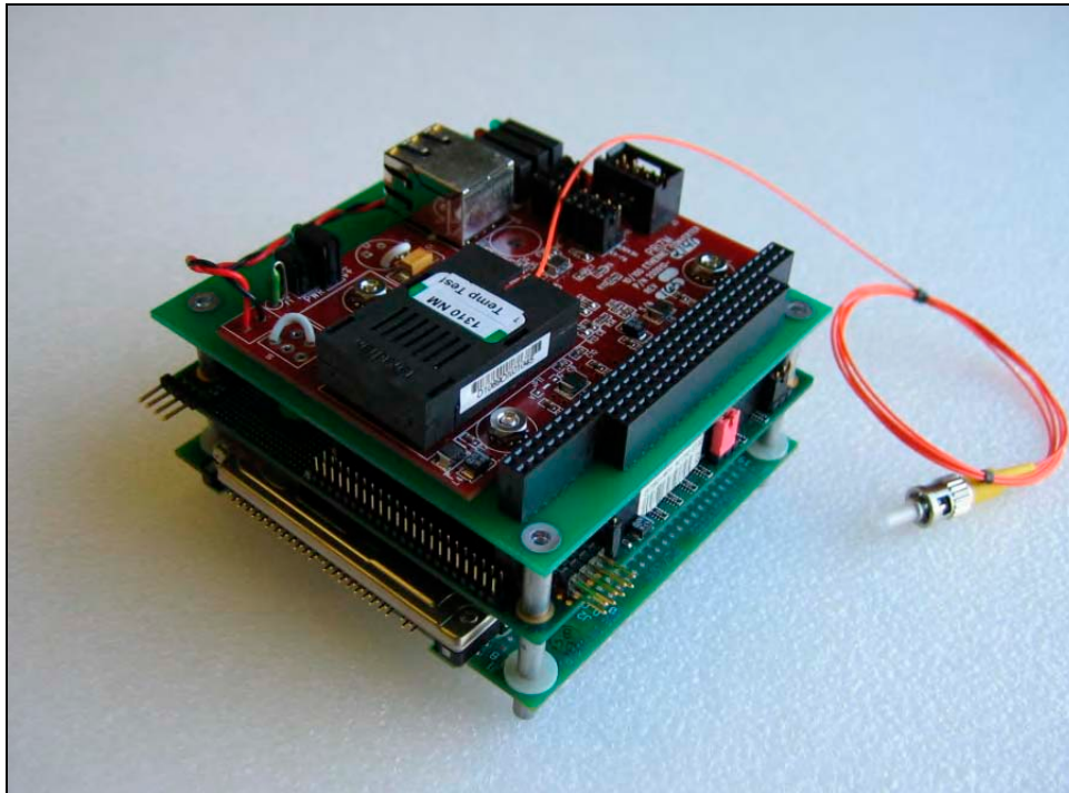
Figure I-4. UUV telemetry component mounting.
