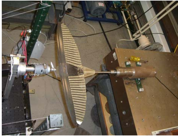
Figure 21. Top View of the Propeller Test Stand (left) and the MAV Testbed Attached to Six-Component Balance (right)
