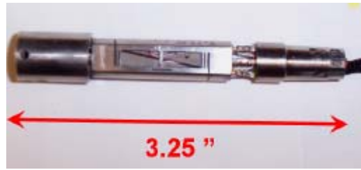
Figure 22. AFIT-1 Six-Component Balance (Rivera Parga 2004:70)
