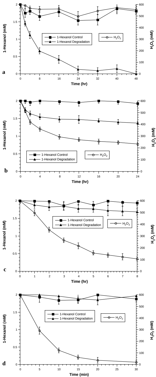
Figure 8.2.1-1. 1-Hexanol and hydrogen peroxide concentrations in manganese (II)-catalyzed CHP reactions (600 mM hydrogen peroxide and 200 mM manganese sulfate). (a) pH 4.0; (b) pH 6.0; (c) pH 6.4; (d) pH 6.8
