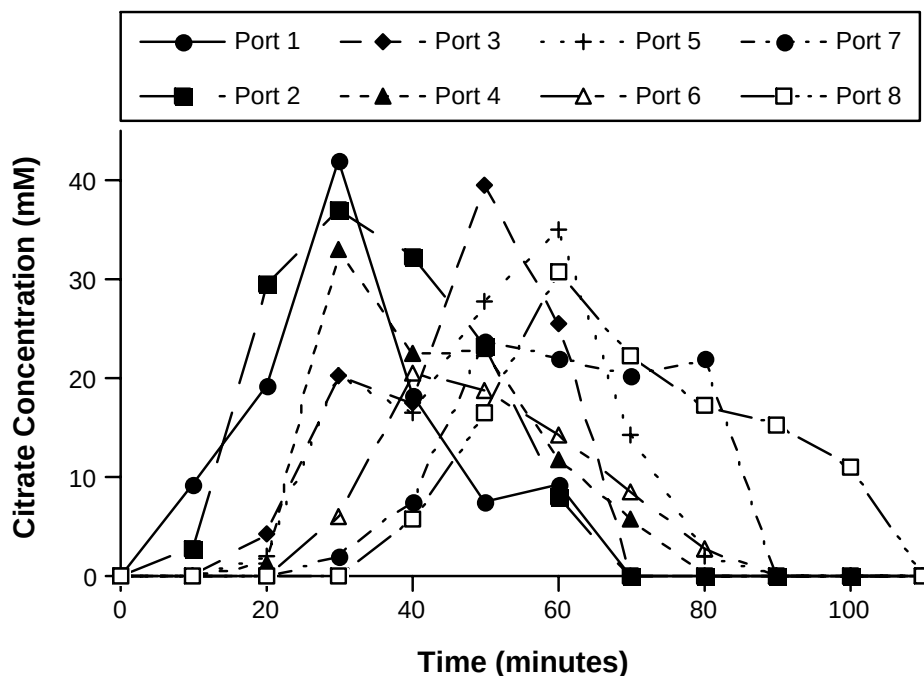
Figure 8.6.6-15. Concentration of citrate in each of eight ports over time in a column of manganese coated sand (MCS) containing hexachlorobenzene (HCB) treated with \text{H}_2\text{O}_2 stabilized by 25 mM citrate at pH 7.
