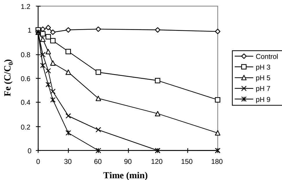
Figure 8.2.2-6. Soluble ( Fe^{2+}/Fe^{3+} ) - NTA concentrations with 294 mM hydrogen peroxide at varying pH
