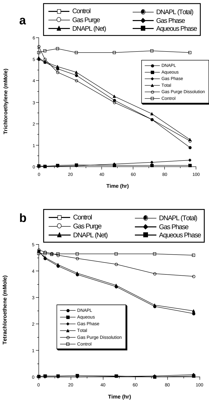
Figure 8.4.4-1. Destruction of (a) TCE and (b) PCE DNAPLs by CHP (5 mM iron (III):HKCH chelate and 2 M hydrogen peroxide at pH 3).
