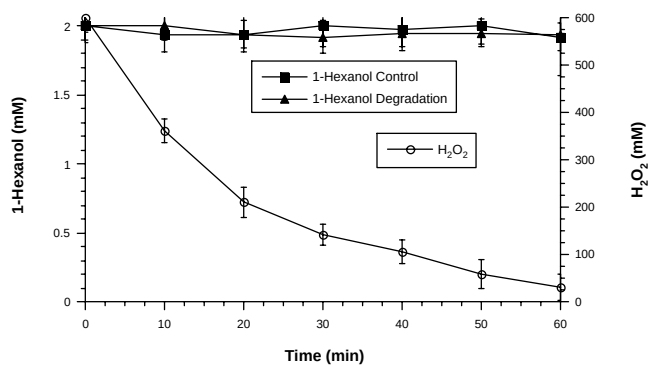
Figure 8.2.1-7. Hexanol and hydrogen peroxide concentrations in CHP reactions catalyzed by pyrolusite (600 mM hydrogen peroxide and 25 mg pyrolusite at pH 6.8)
