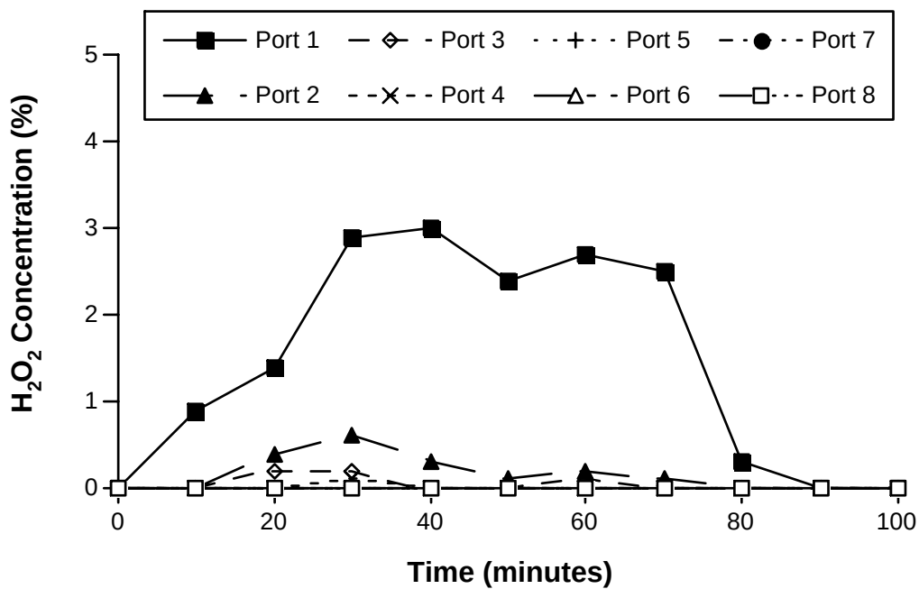
Figure 8.6.6-3. Decomposition of unstabilized \text{H}_2\text{O}_2 in a column of iron coated sand (ICS) at pH 7.
