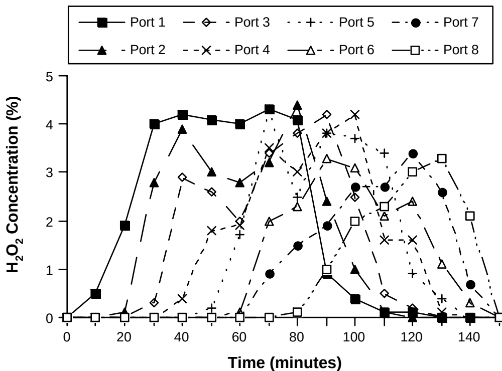
Figure 8.6.6-4. Decomposition of \text{H}_2\text{O}_2 stabilized by 25 mM phytate in a column of iron coated sand (ICS) at pH 7.
