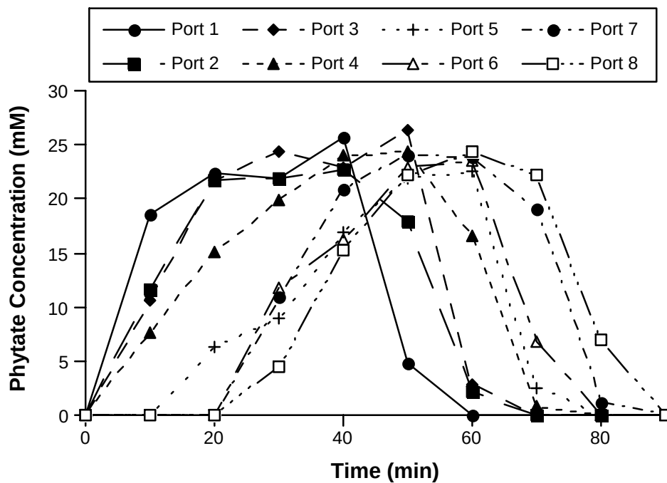
Figure 8.6.6-16. Concentration of phytate in each of eight ports over time in a column of manganese coated sand (MCS) containing hexachlorobenzene (HCB) treated with \text{H}_2\text{O}_2 stabilized by 25 mM phytate at pH 7.
