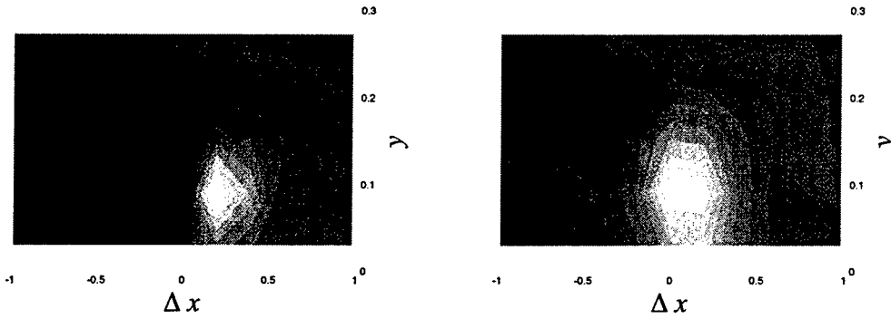
Figure 5.7: Wall-normal spatial distribution of the correlation coefficients for u' : coefficients for \phi^u (left) and \phi^w (right) at \Delta z = 0 . The scale range is \pm 0.046 for \phi^u and \pm 0.36 for \phi^w , with white being a large positive value and black a large negative value. The domain is \pm 5 points in the streamwise direction and 5 points in the wall-normal direction.
