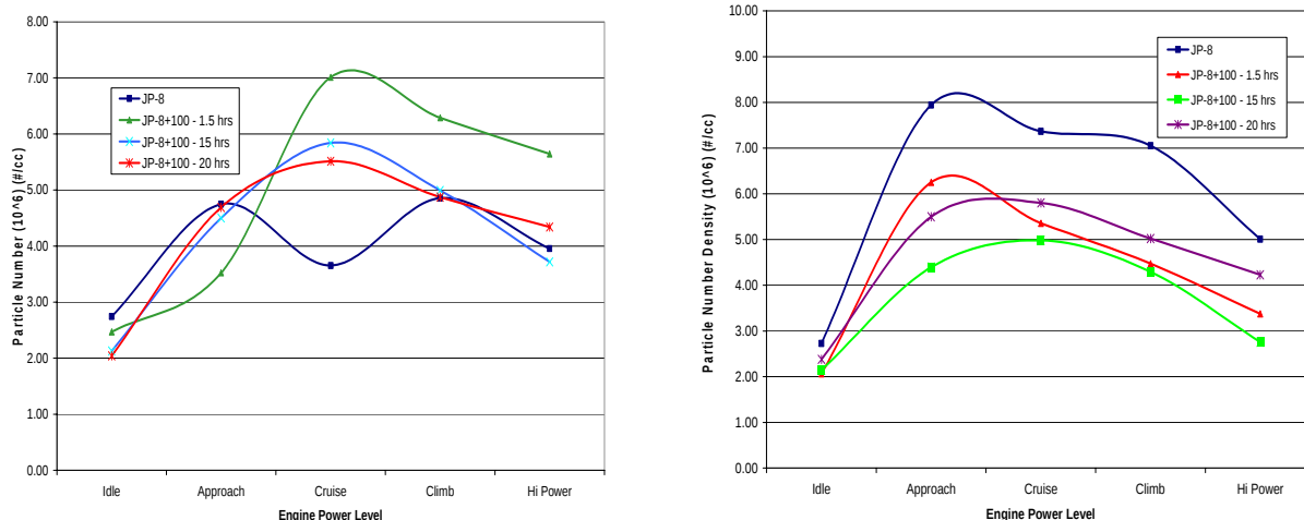
Figure 4.2. PND as a Function of Power Setting for T-43 Engines 607 and 613.
