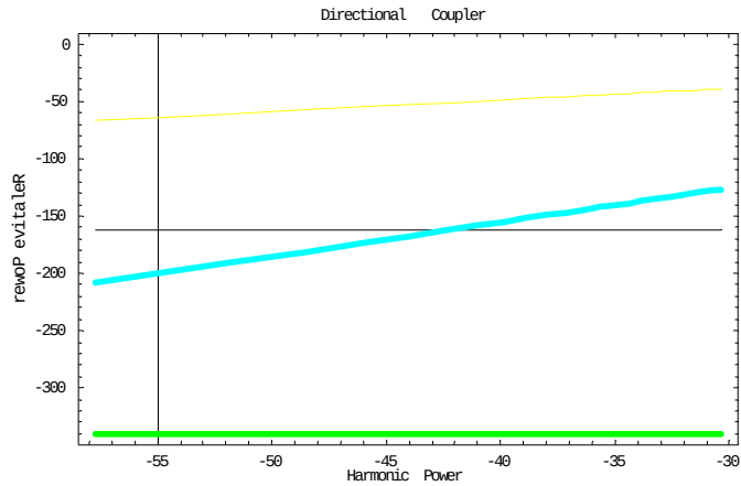
Figure 46: SFDR Calculation Splayed Directional Coupler
