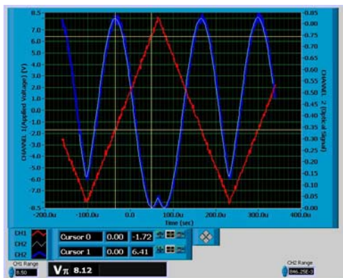
Figure 54: V pi was \sim 8\text{ V} for the 21% chromophore concentration under \sim 60\text{ V}/\mu\text{m} poling conditions.
