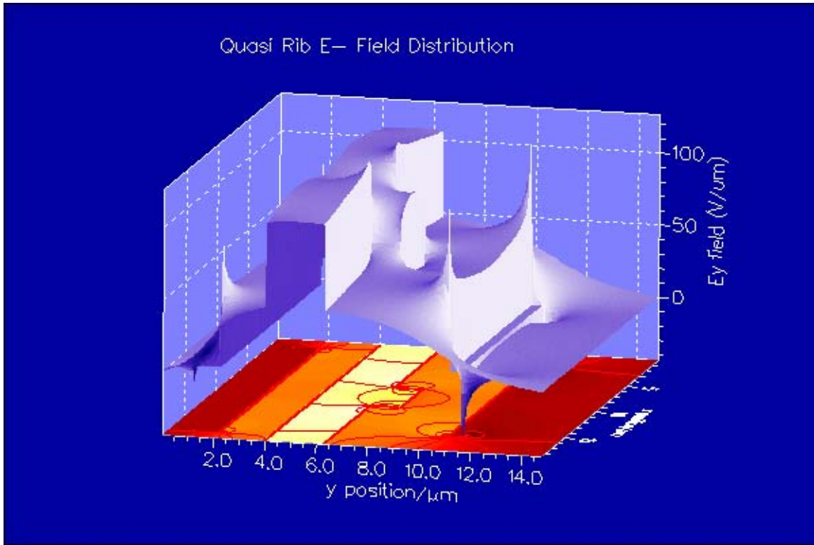
Figure 32: 3-D view of E_y Field: 80-105 V/\mu m across core with 600V applied In this waveguide polymer stack model. The field across the core is \sim 105 V/\mu m in the non-trench area and \sim 85 V/\mu m in the waveguide trench area. Note the edge singularities are also approaching 100 V/\mu m .
