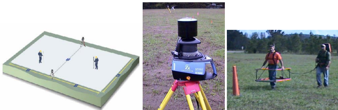
Figure 2-6. ArcSecond Constellation System.
