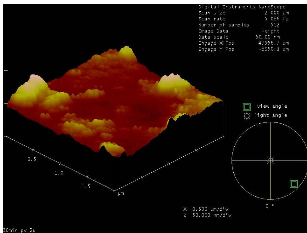
Figure 66. Atomic Force Microscopy surface roughness and 3-D profile for the CNT film grown at 1700°C under 10^{-3} Torr vacuum for 0.5-hours and with no post-growth annealing.
