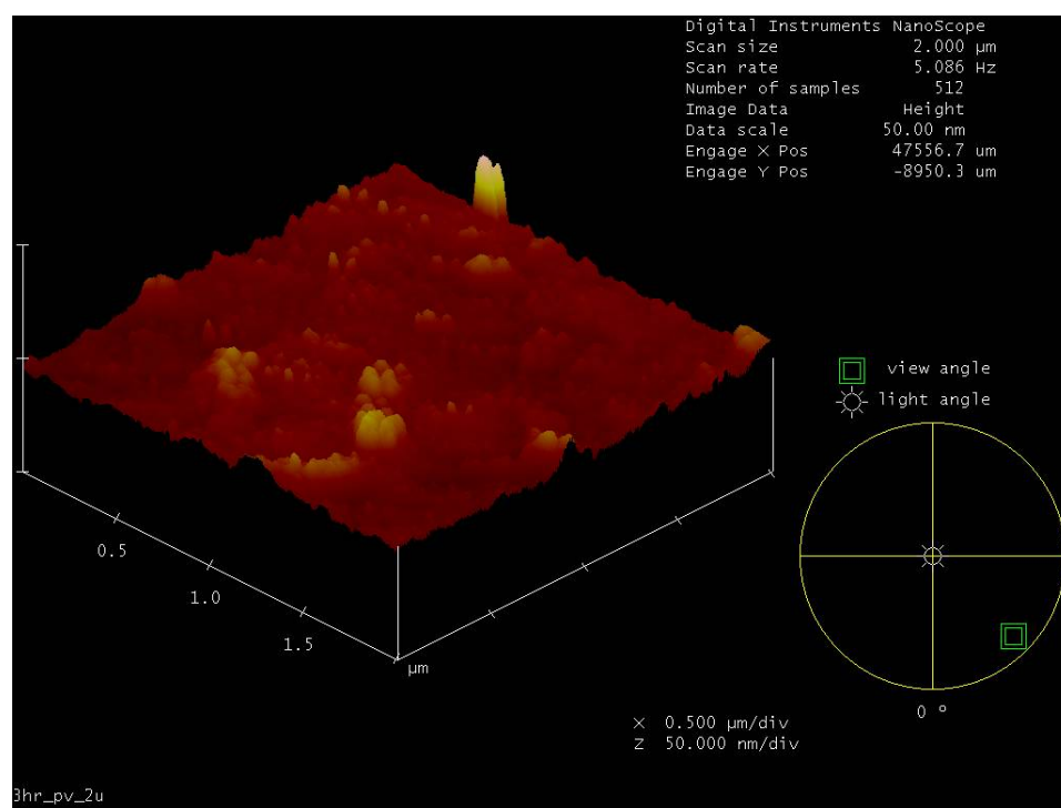
Figure 70. Atomic Force Microscopy surface roughness and 3-D profile for the CNT film grown at 1700°C under 10^{-3} Torr vacuum for 3-hours and with no post-growth annealing.
