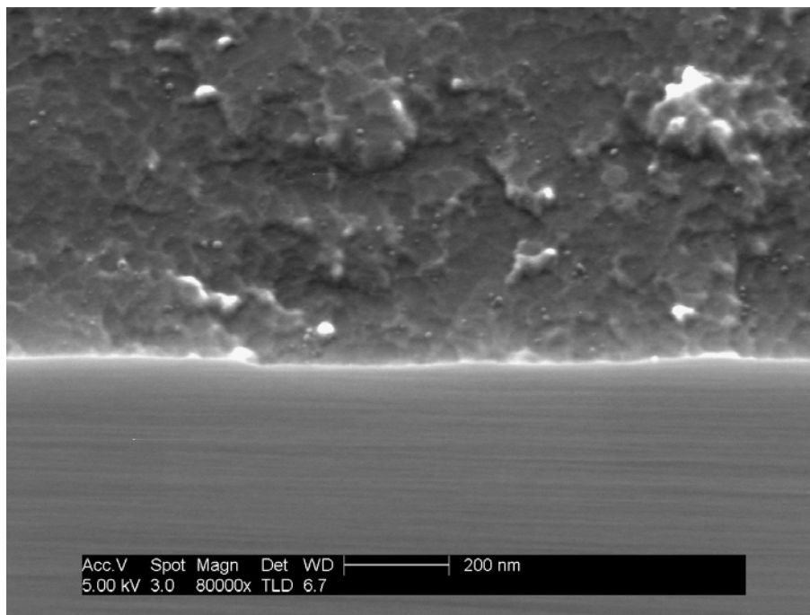
Figure 41. C-face CNTs grown at 1700°C under 10^{-5} Torr vacuum for 1-hour, after a 10-minute anneal at 620°C in flowing O 2 , 30° tilt, 80,000x magnification.
