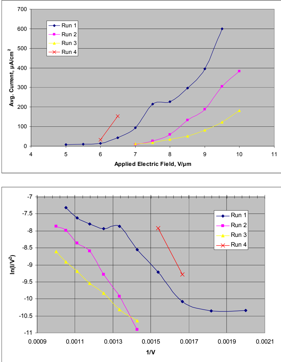
Figure 56. Field emission data for the CNT film grown at 1700^\circ\text{C} under 10^{-5} Torr vacuum for 3-hours and with no post-growth annealing.
