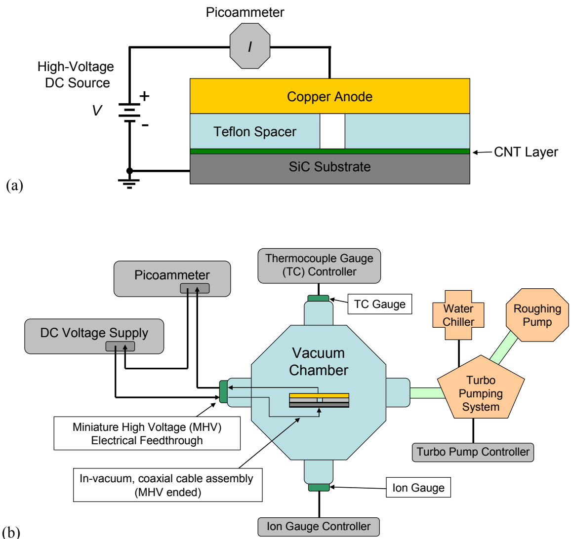
Figure 3. Illustrations of the: (a) vacuum tube diode test setup, and (b) overall test setup.
