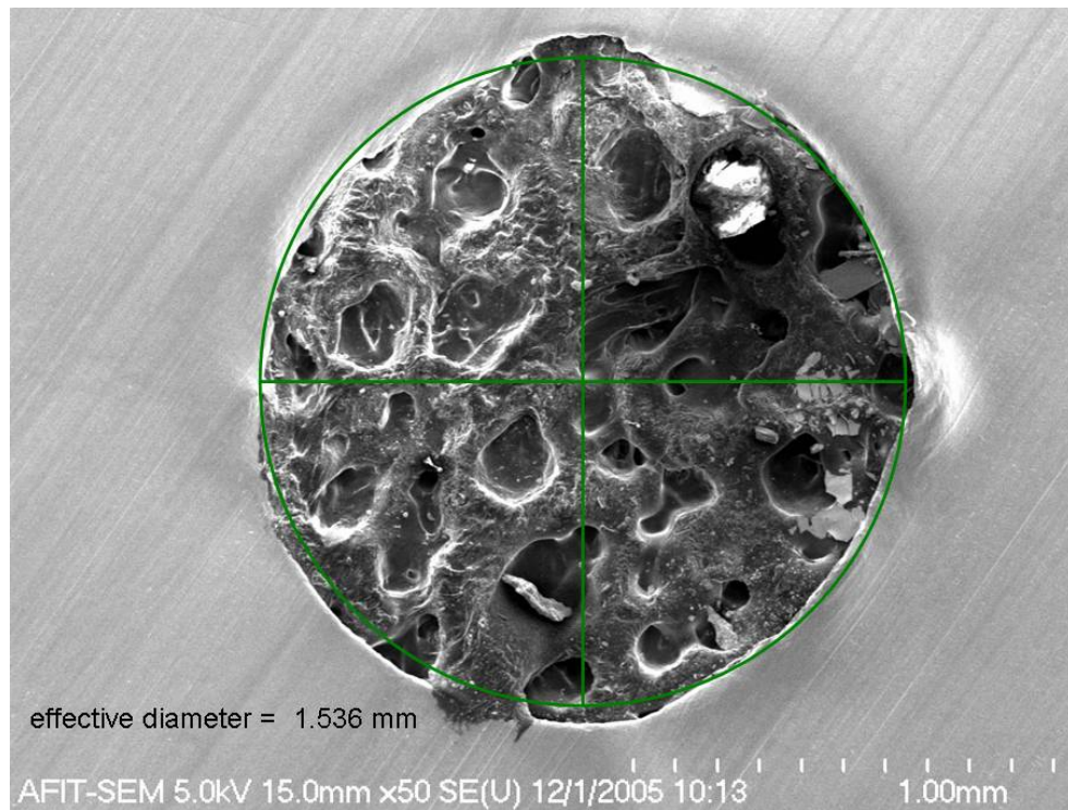
Figure 28. SEM image of the 1/16" hole made using the punch tool.
