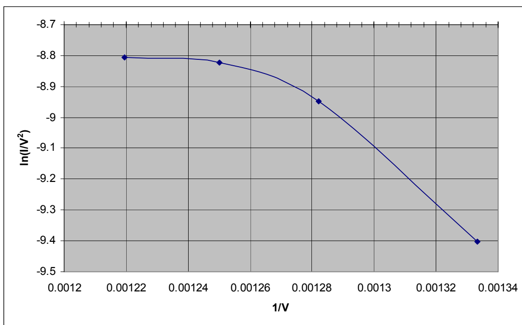
Figure 52. Data collected for 1 run on the CNT film grown at 1700°C under 10^{-5} Torr vacuum for 0.5-hours and annealed for 10-minutes at 620°C in flowing O_2 .
