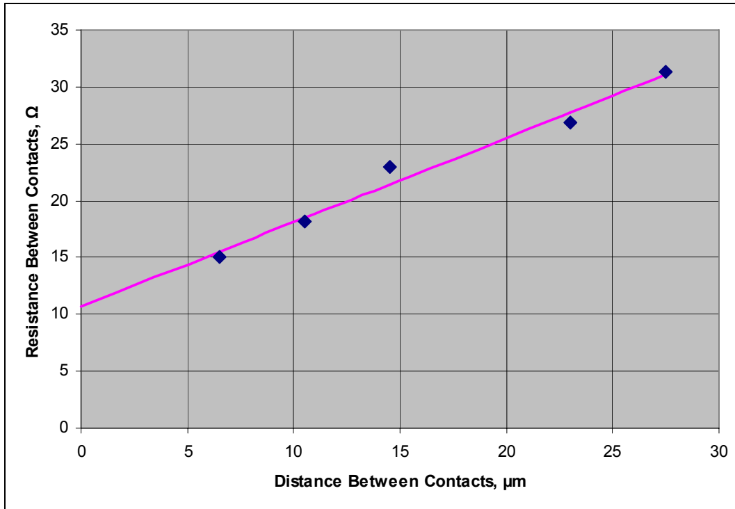
Figure 37. TLM data giving measured resistance between pads versus pad separation and the least squares fit to the measured data (0.5-hour anneal at 1700°C and 10^{-3} Torr).
