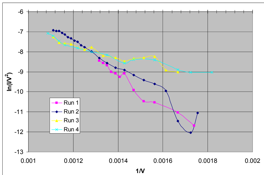
Figure 53. Field emission data for the CNT film grown at 1700°C under 10^{-3} Torr vacuum for 0.5-hours and annealed for 10-minutes at 620°C in flowing \text{O}_2 .
