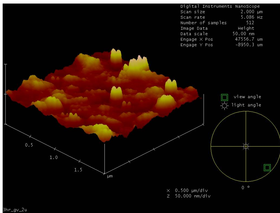
Figure 69. Atomic Force Microscopy surface roughness and 3-D profile for the CNT film grown at 1700°C under 10^{-5} Torr vacuum for 3-hours and with no post-growth annealing.
