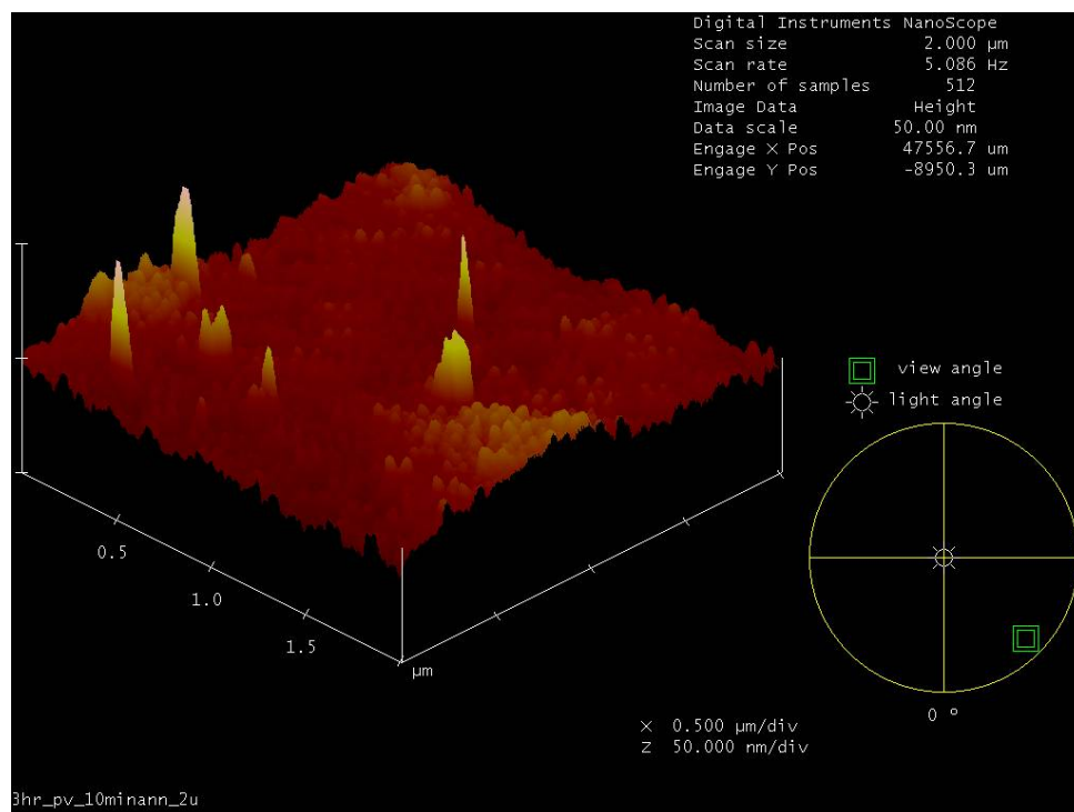
Figure 72. Atomic Force Microscopy surface roughness and 3-D profile for the CNT film grown at 1700°C under 10^{-3} Torr vacuum for 3-hours and annealed for 10-minutes at 620°C in flowing O 2 .
