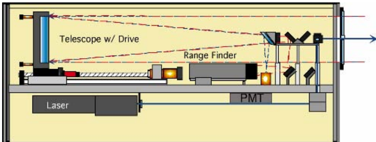
Figure B-3. Schematic of Optical Layout for the Reconfigured MRLS Unit. Reconfiguration Involved the Replacement of a Spectrometer/ICCD Detection Subsystem with a Single-Element PMT
