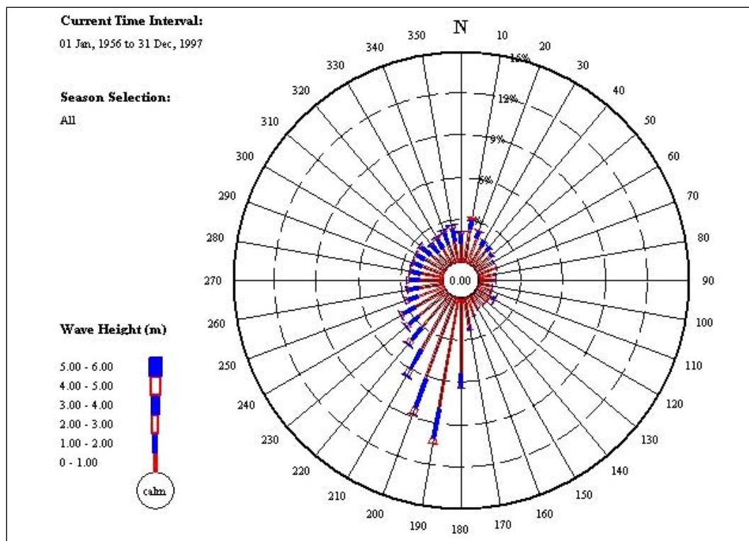
Figure B4. Wave height rose, Portage Lake, MI.
