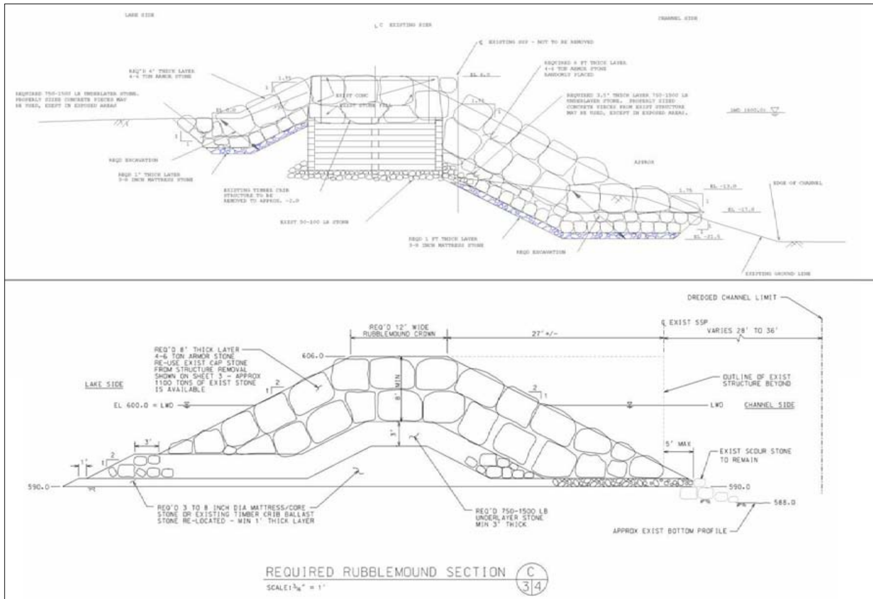
Figure A6. Ontonagon Harbor, MI.
