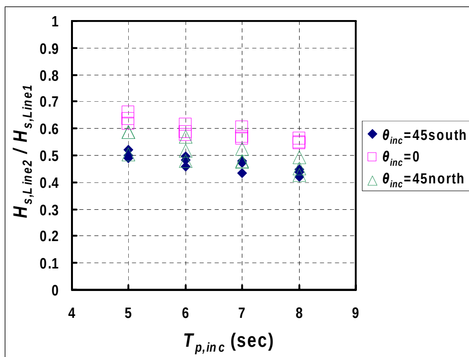
Figure 23. Effect of T_p and wave direction on pocket absorber performance, existing condition, swl = 0 LWD.
