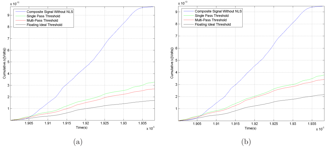
Figure 4.3: Cumulative point-by-point |\Delta| for all thresholding techniques. (a) Average Input \frac{P_u}{P_a} = -0.10\text{dB} (b) Average Input \frac{P_u}{P_a} = 2.88\text{dB}
