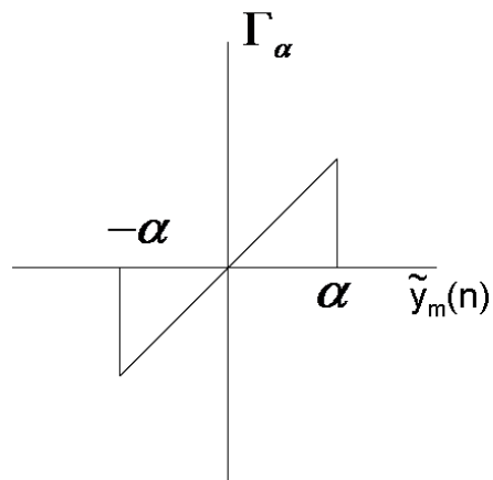
Figure 2.5: Hole-punch nonlinearity. When |\tilde{y}_m[n]| > \alpha , \tilde{y}_m[n] is set to zero.
