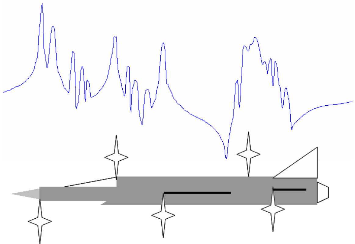
Figure 3.21: RCS Range Profile and Corresponding Scattering Locations for Measurement Target
