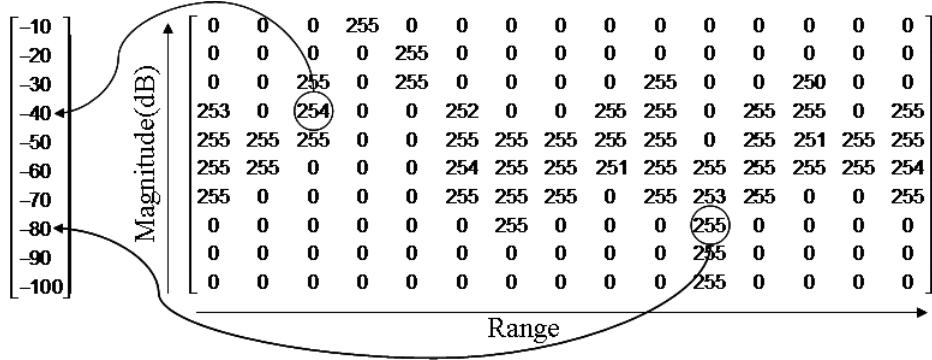
Figure 3.17: Mapping Technique for Data Image Matrix
