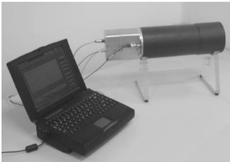
FIGURE 7. Photograph of xenon detector arrangement
