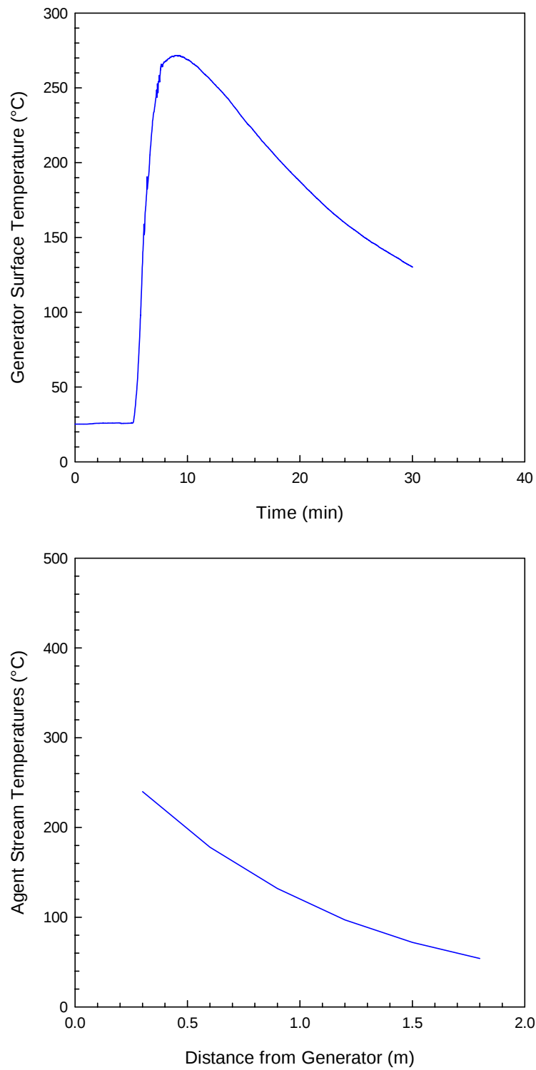
Figure 21. System Two Generator Surface and Agent Stream Temperatures.
