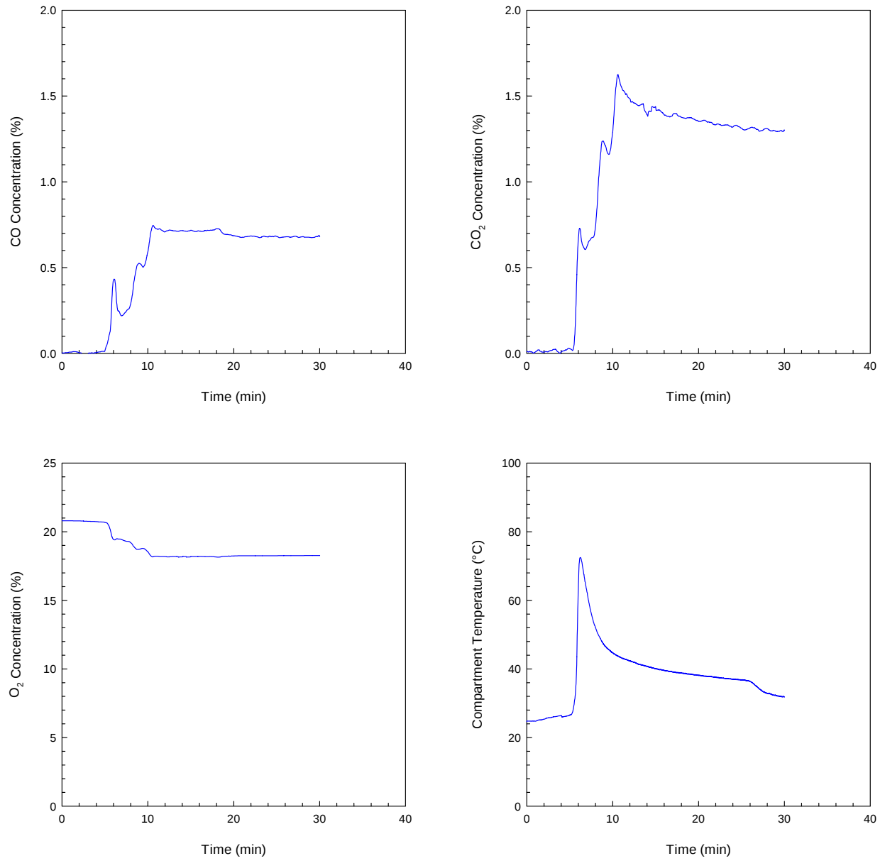
Figure 19. System Two Compartment Conditions.
