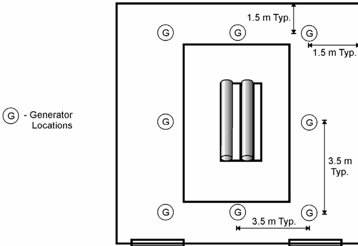
Figure 8. AES Generator Locations.
