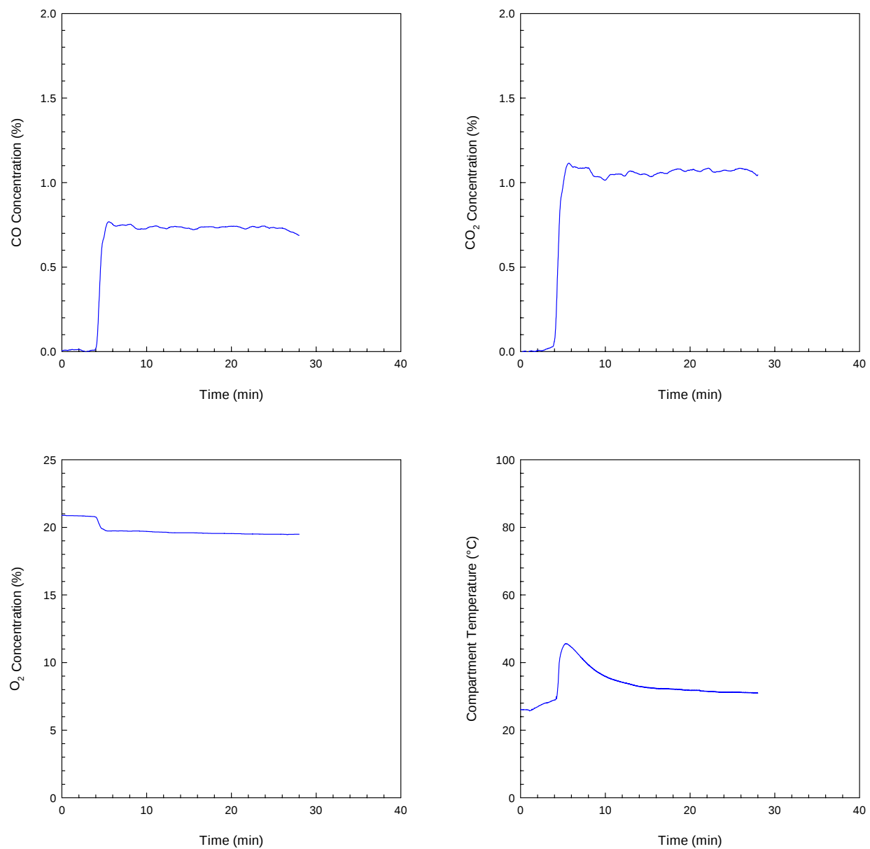
Figure 23. System Three Compartment Conditions.
