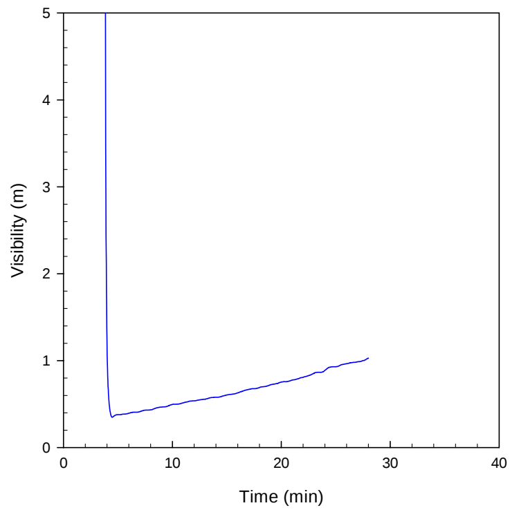
Figure 24. System Three Particulate Density and Visibility.
