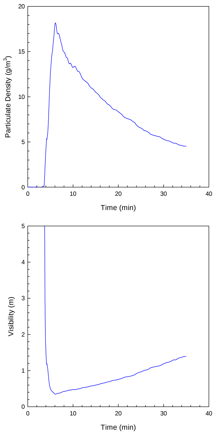
Figure 16. System One Particulate Density and Visibility.
