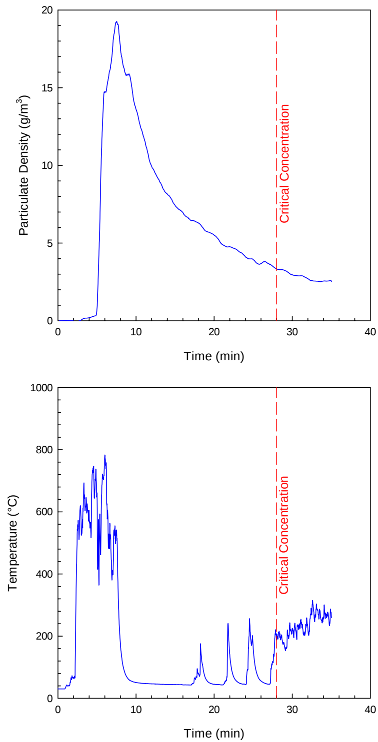
Figure 22. System Two Reignition Test Results.
