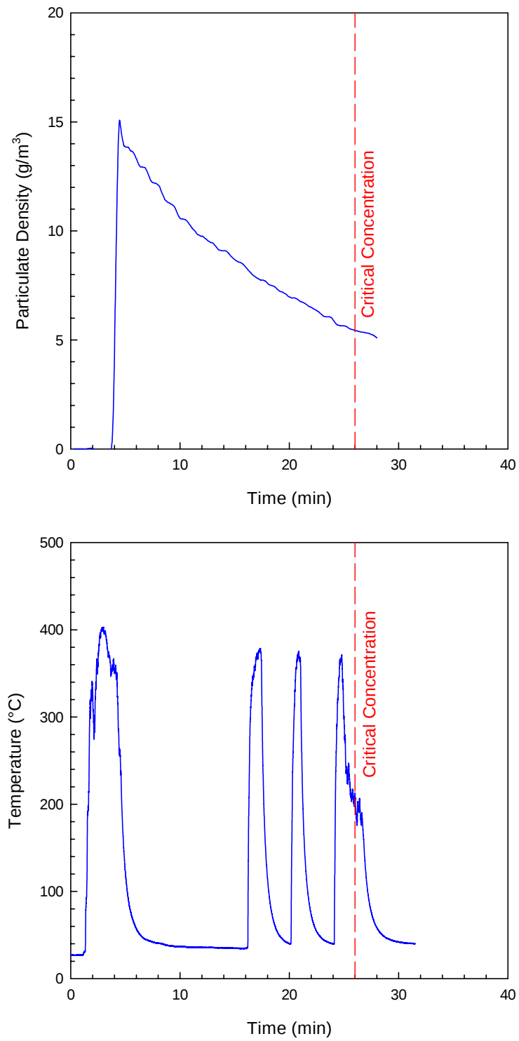
Figure 26. System Three Reignition Test Results.
