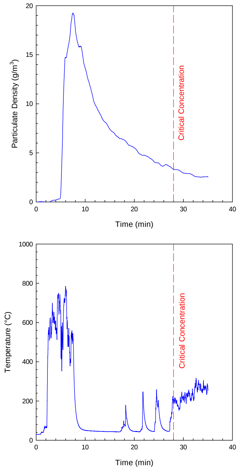
Figure 14. Critical Extinguishing Concentration (System Two).
