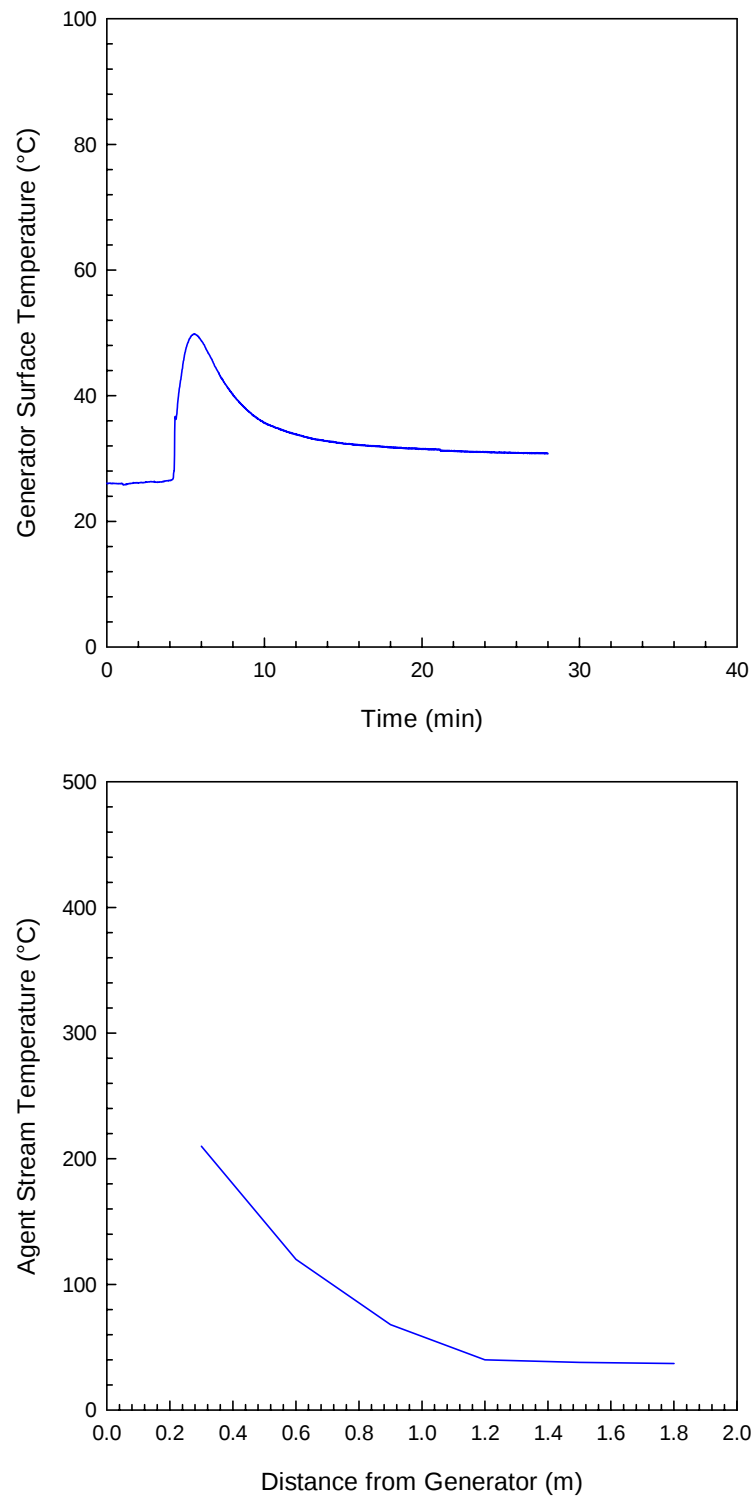
Figure 25. System Three Generator Surface and Agent Stream Temperatures.
