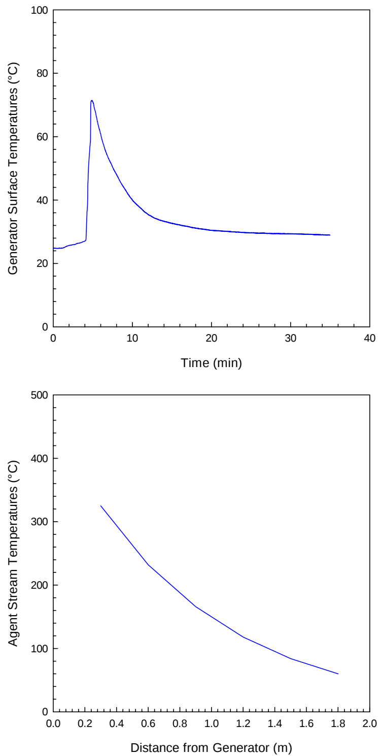
Figure 17. System One Generator Surface and Agent Stream Temperatures.
