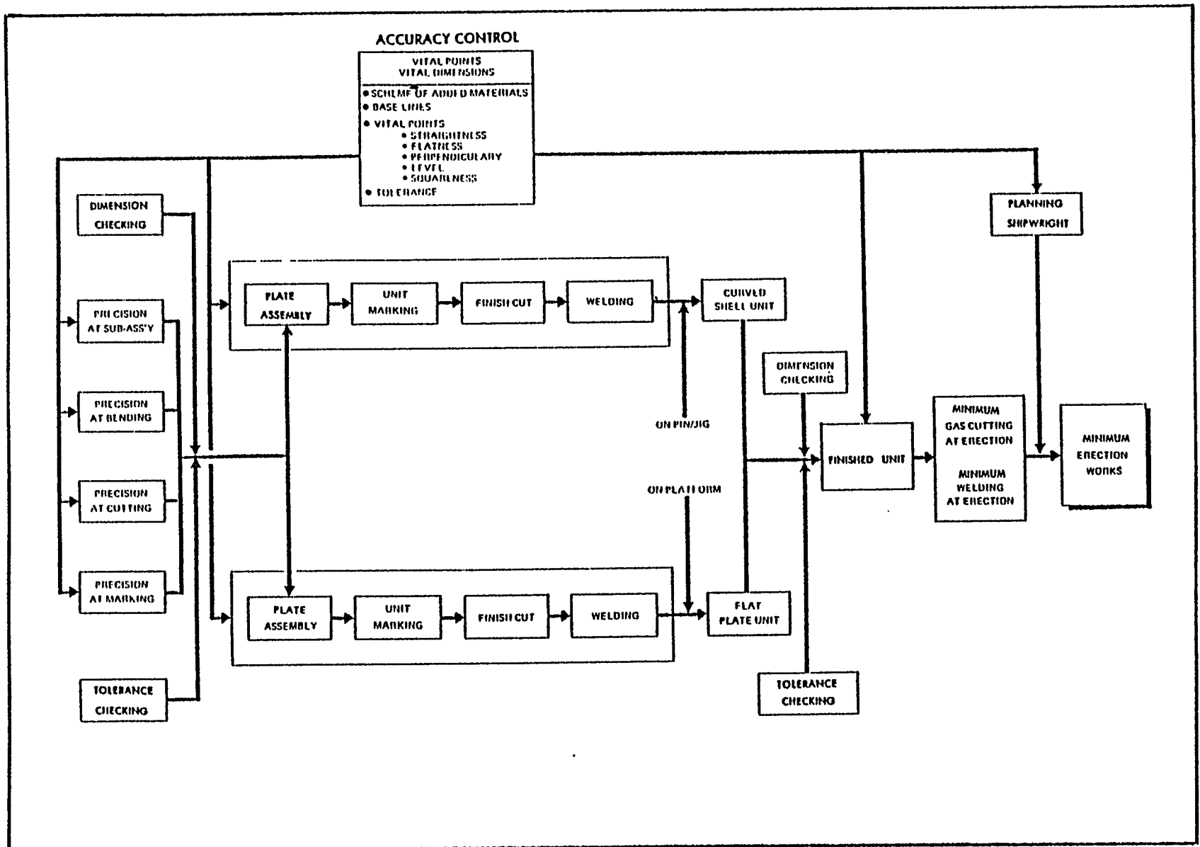
CONCEPT OF ACCURACY CONTROL IN TWT
