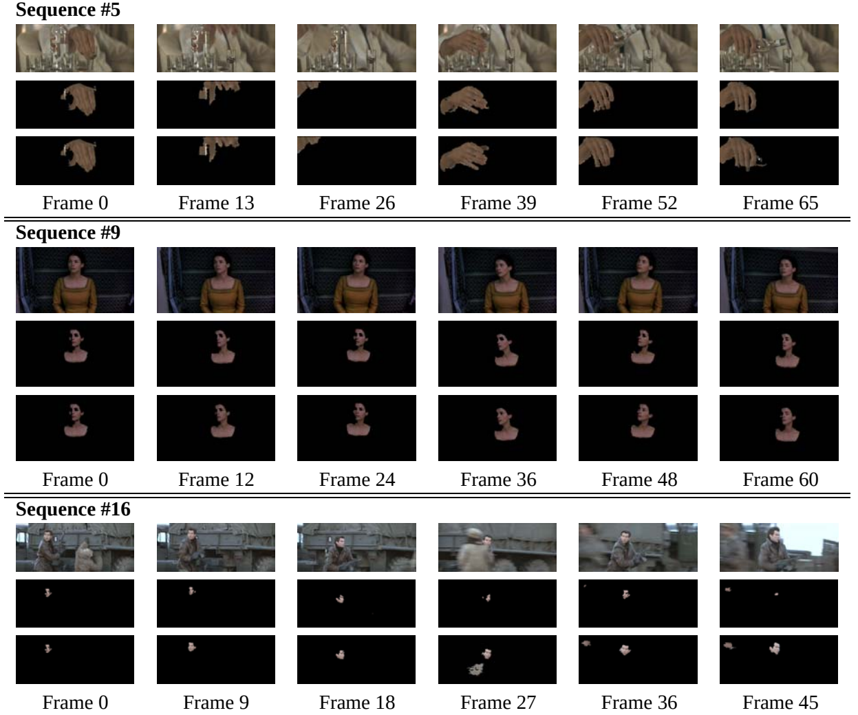
Figure 12: Examples of segmentation obtained by the dynamic and static approaches. The examples above are among those for which our system had a superior performance. Frames from image sequence (top), static segmentation (middle), and dynamic segmentation (bottom) are shown.
