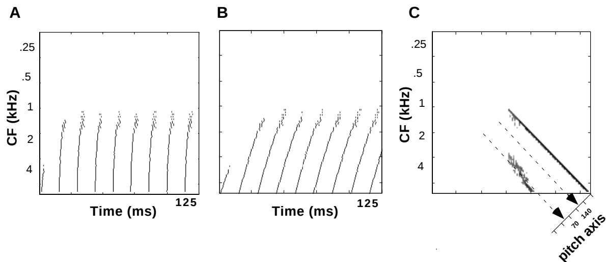
Figure 8: Measuring repetition pitch with the coincidence matrix. A: The synchronized responses to a stimulus consisting of 10^{th} – 110^{th} harmonics of 70 Hz. B: The synchronized waves are “tilted” by a gradual increase in latency from high to low CF channels. C: The average output of the coincidence matrix shows a strong line of coincidences parallel to the diagonal, and at a distance that reflects the repetition period of the stimulus. Faster rates cause this line to move gradually closer to the main diagonal.
